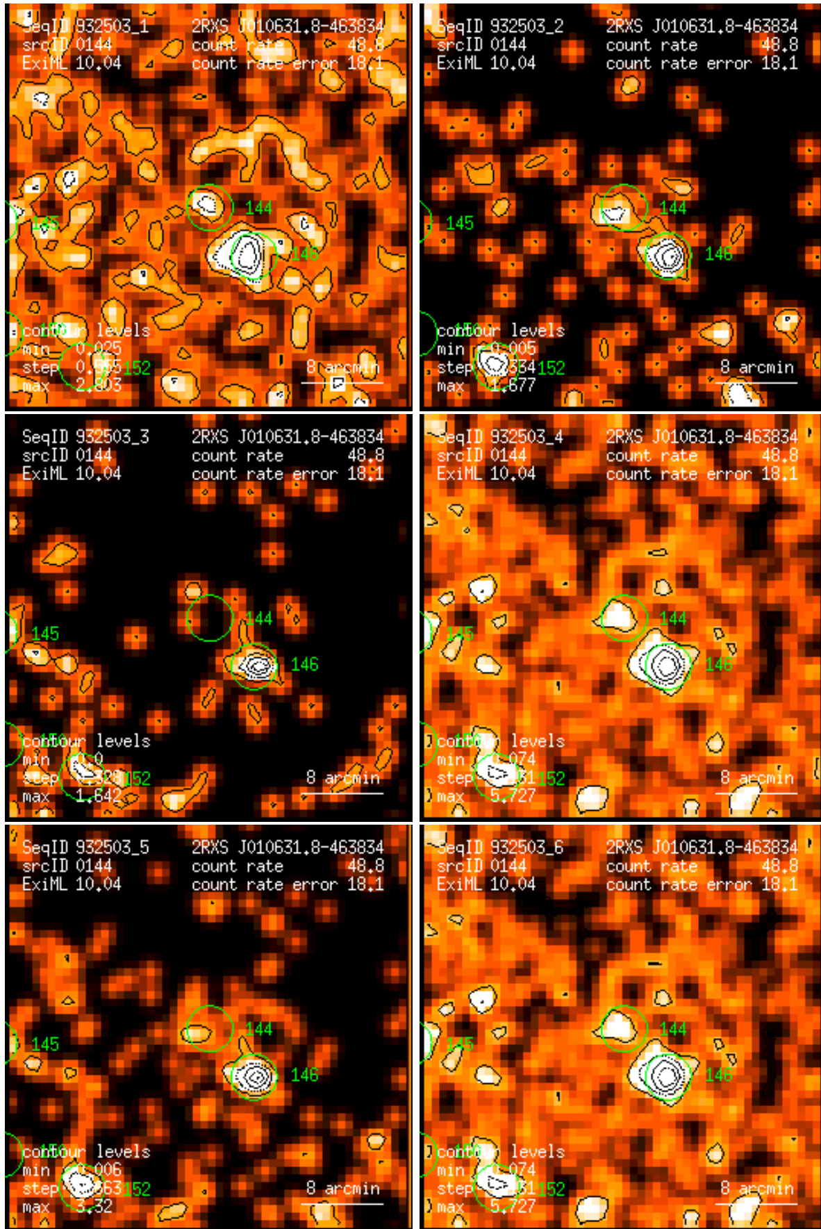
Figure 144: RASS 932503: detection 0144: band rate images, Gaussian filter: (1) PSPC channels 11 – 41, (2) 52 – 90, (3) 91 – 201, (4) 11 – 235, (5) 52 – 201, (6) 11 – 201. Broad band rates in counts/ks. Band rate contour levels in counts/ks/arcmin 2 .
