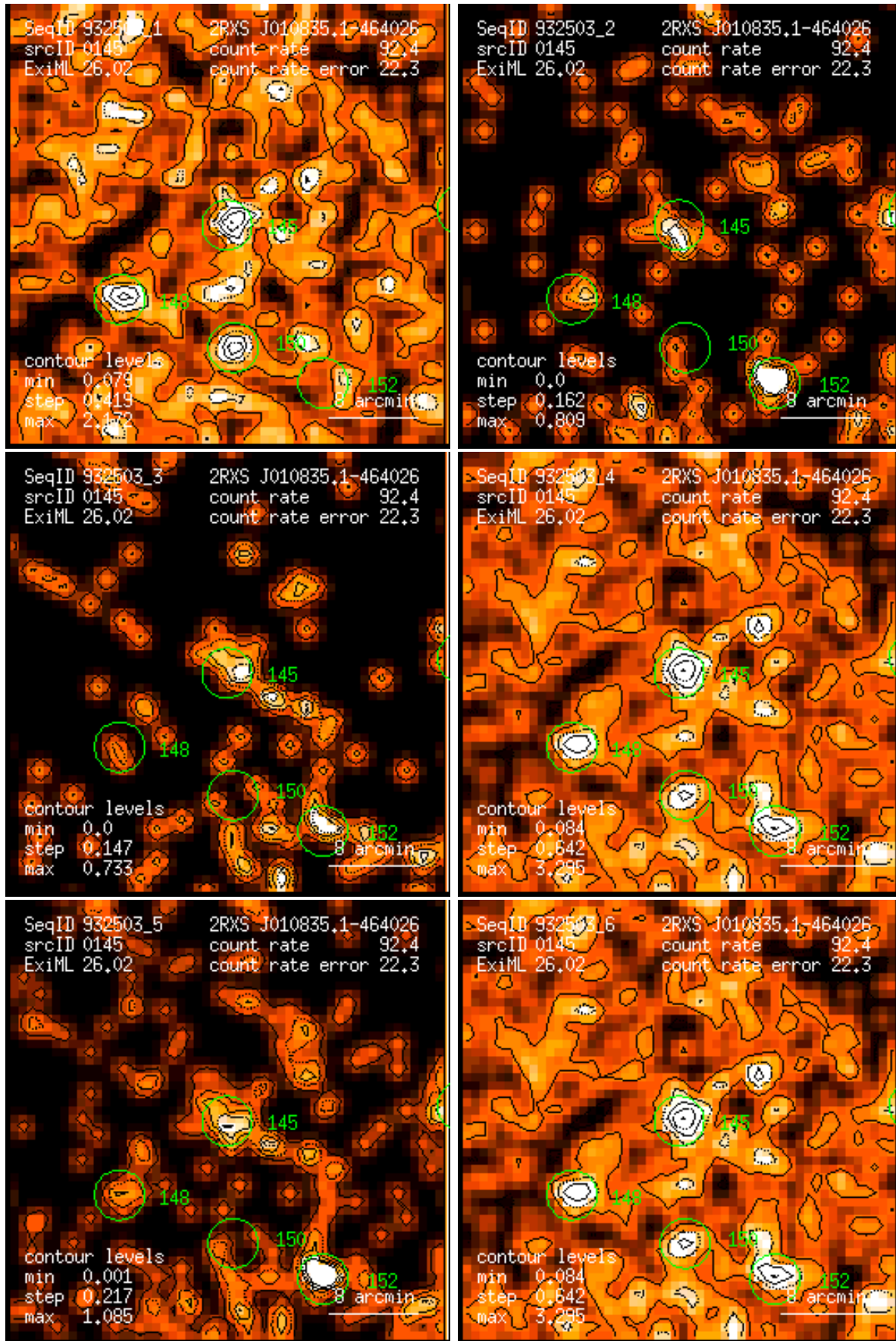
Figure 145: RASS 932503: detection 0145: band rate images, Gaussian filter: (1) PSPC channels 11 – 41, (2) 52 – 90, (3) 91 – 201, (4) 11 – 235, (5) 52 – 201, (6) 11 – 201. Broad band rates in counts/ks. Band rate contour levels in counts/ks/arcmin 2 .
