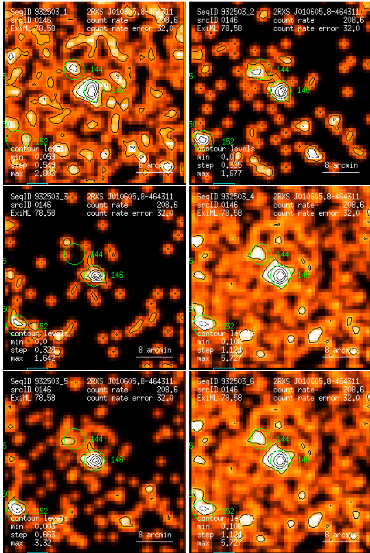
Figure 146: RASS 932503: detection 0146: band rate images, Gaussian filter: (1) PSPC channels 11 – 41, (2) 52 – 90, (3) 91 – 201, (4) 11 – 235, (5) 52 – 201, (6) 11 – 201. Broad band rates in counts/ks. Band rate contour levels in counts/ks/arcmin 2 .
