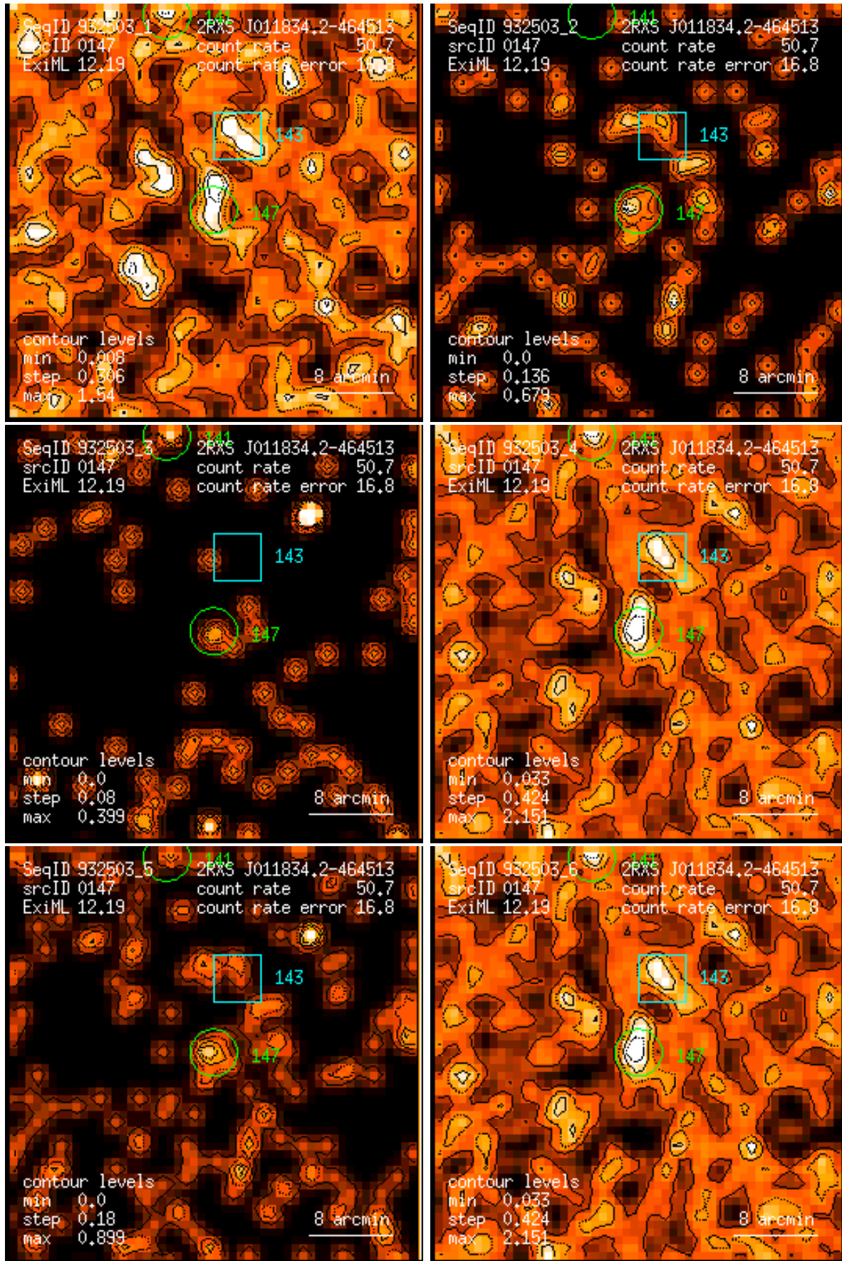
Figure 147: RASS 932503: detection 0147: band rate images, Gaussian filter: (1) PSPC channels 11 – 41, (2) 52 – 90, (3) 91 – 201, (4) 11 – 235, (5) 52 – 201, (6) 11 – 201. Broad band rates in counts/ks. Band rate contour levels in counts/ks/arcmin 2 .
