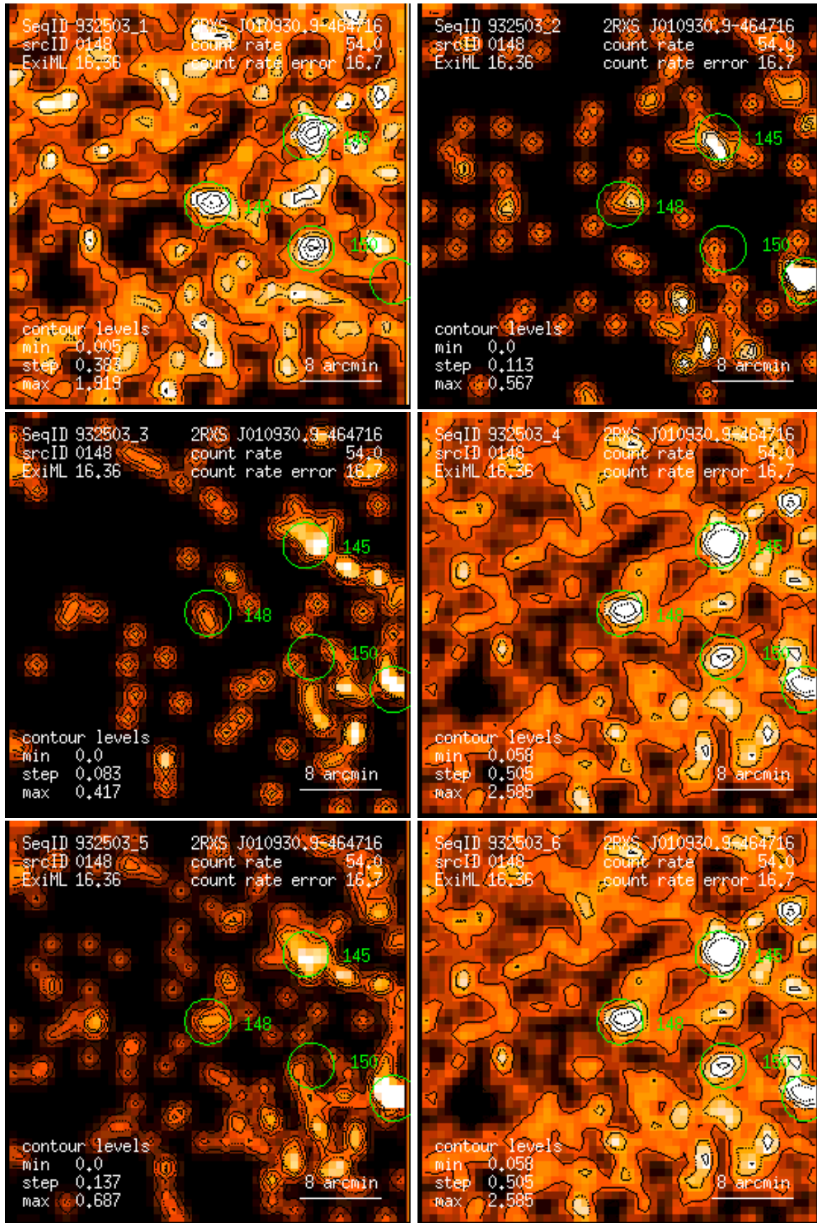
Figure 148: RASS 932503: detection 0148: band rate images, Gaussian filter: (1) PSPC channels 11 – 41, (2) 52 – 90, (3) 91 – 201, (4) 11 – 235, (5) 52 – 201, (6) 11 – 201. Broad band rates in counts/ks. Band rate contour levels in counts/ks/arcmin 2 .
