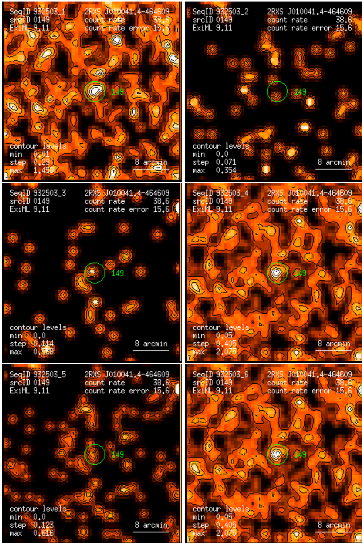
Figure 149: RASS 932503: detection 0149: band rate images, Gaussian filter: (1) PSPC channels 11 – 41, (2) 52 – 90, (3) 91 – 201, (4) 11 – 235, (5) 52 – 201, (6) 11 – 201. Broad band rates in counts/ks. Band rate contour levels in counts/ks/arcmin 2 .
