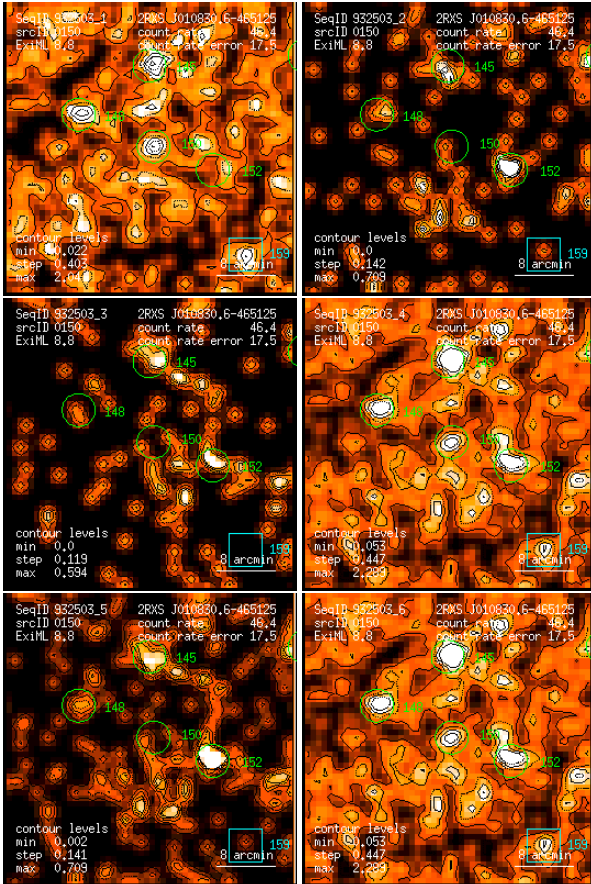
Figure 150: RASS 932503: detection 0150: band rate images, Gaussian filter: (1) PSPC channels 11 – 41, (2) 52 – 90, (3) 91 – 201, (4) 11 – 235, (5) 52 – 201, (6) 11 – 201. Broad band rates in counts/ks. Band rate contour levels in counts/ks/arcmin 2 .
