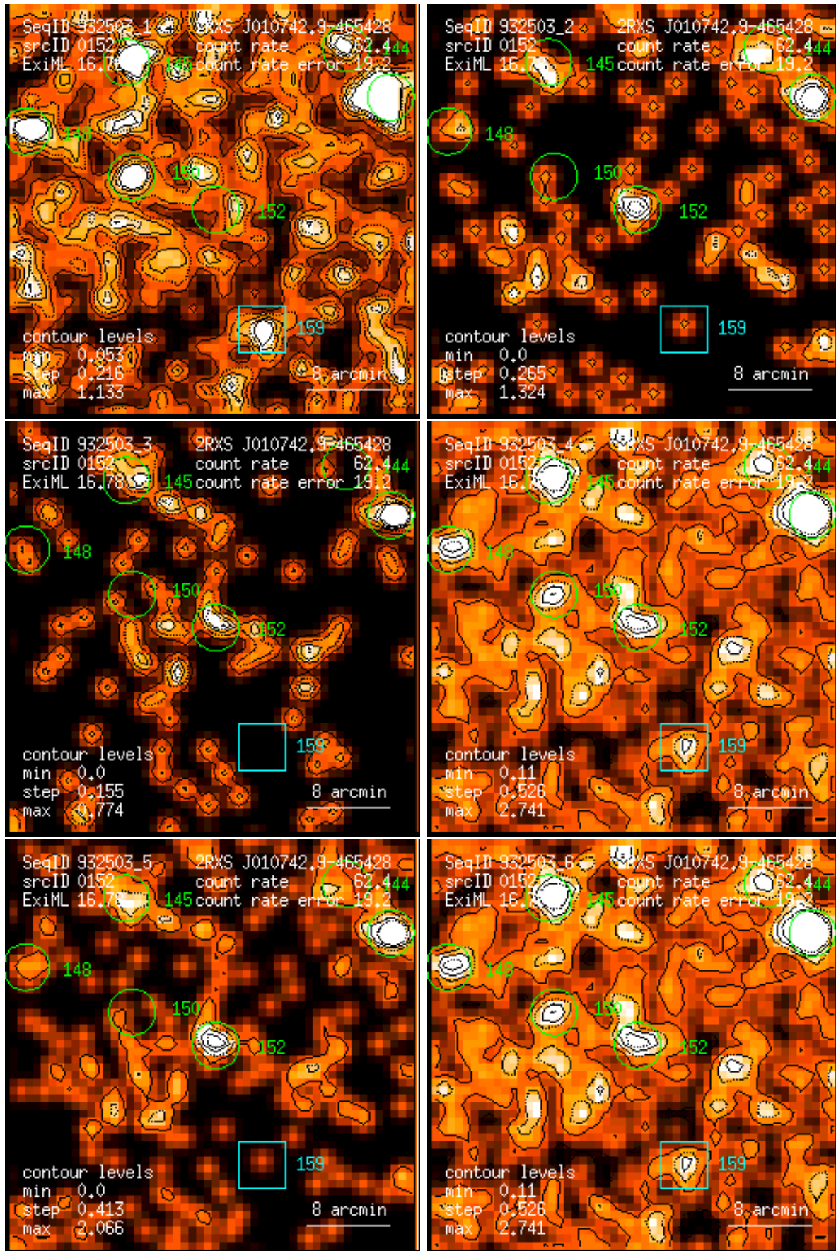
Figure 152: RASS 932503: detection 0152: band rate images, Gaussian filter: (1) PSPC channels 11 – 41, (2) 52 – 90, (3) 91 – 201, (4) 11 – 235, (5) 52 – 201, (6) 11 – 201. Broad band rates in counts/ks. Band rate contour levels in counts/ks/arcmin 2 .
