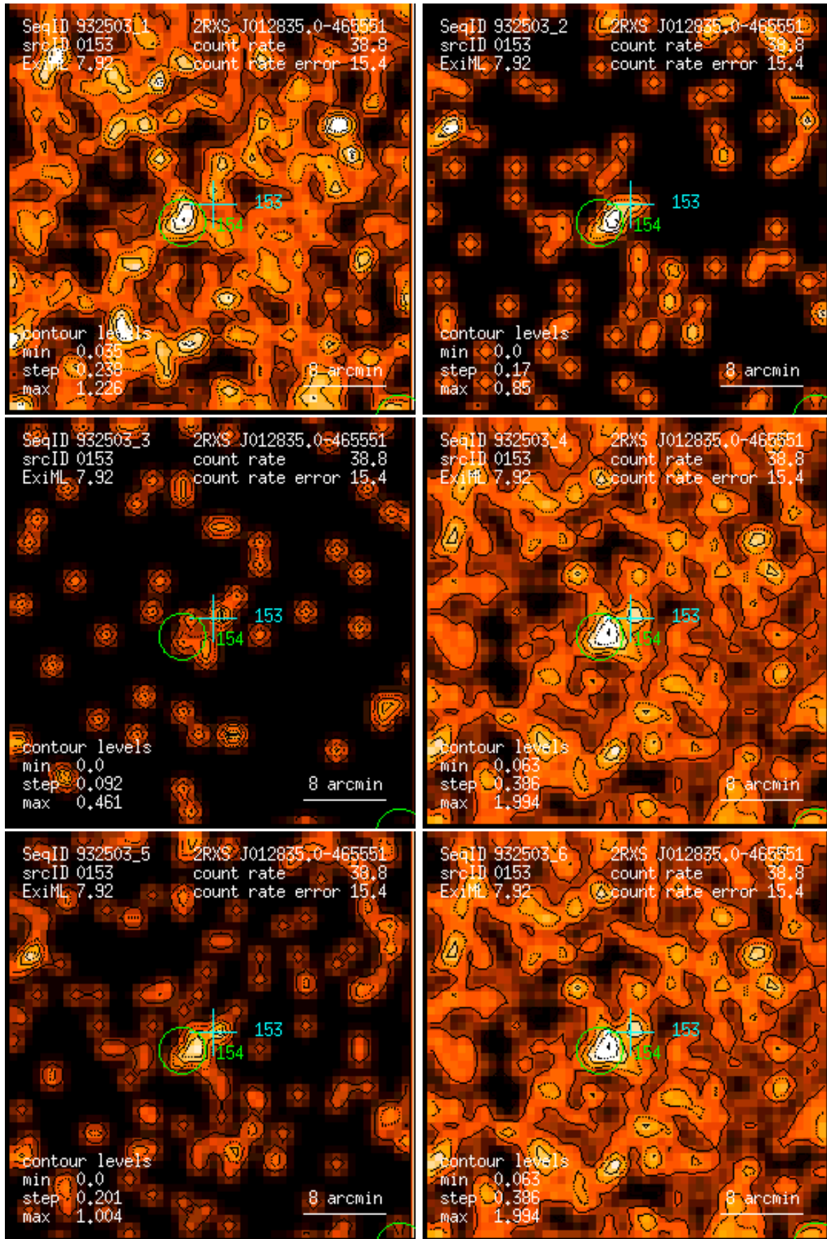
Figure 153: RASS 932503: detection 0153: band rate images, Gaussian filter: (1) PSPC channels 11 – 41, (2) 52 – 90, (3) 91 – 201, (4) 11 – 235, (5) 52 – 201, (6) 11 – 201. Broad band rates in counts/ks. Band rate contour levels in counts/ks/arcmin 2 .
