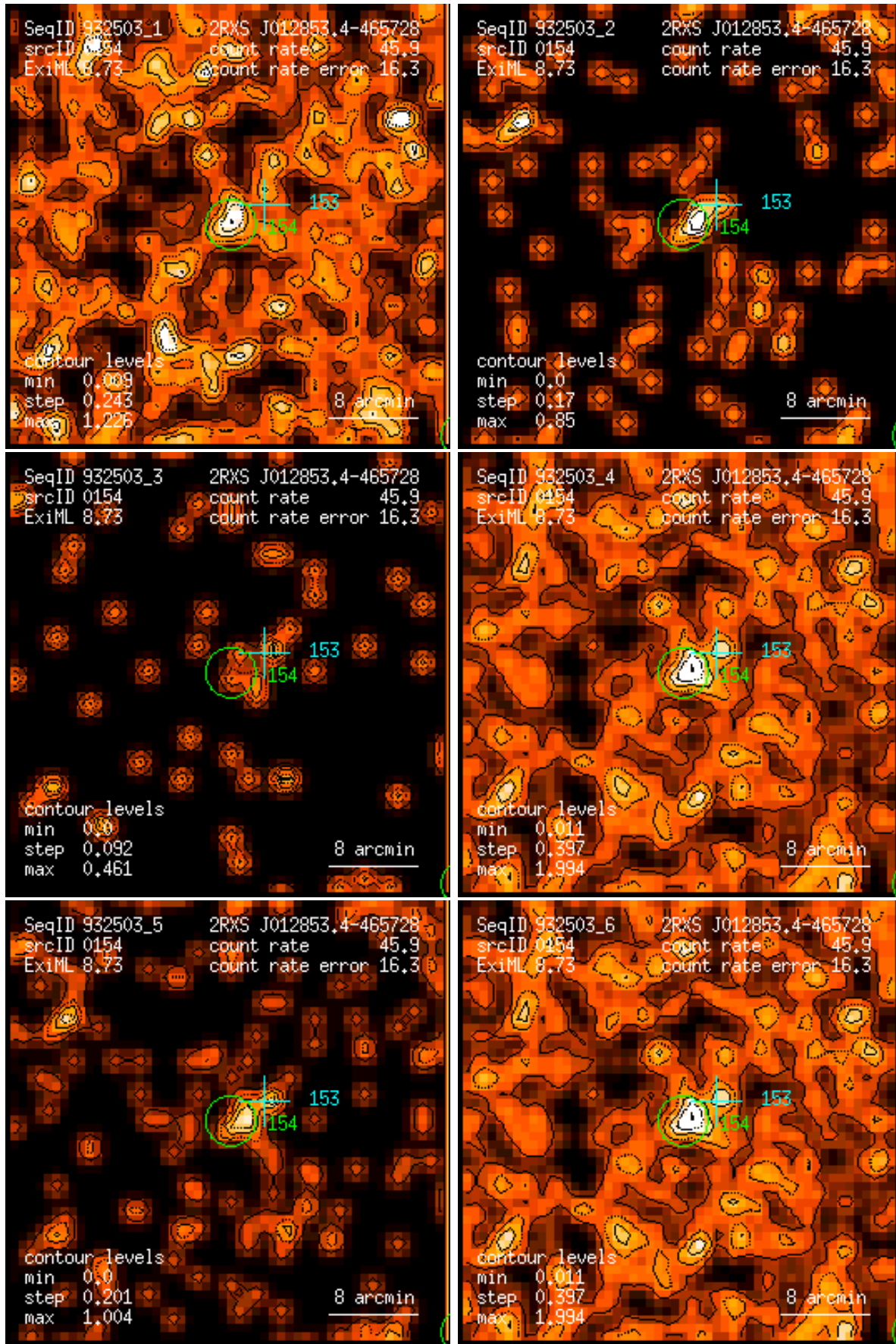
Figure 154: RASS 932503: detection 0154: band rate images, Gaussian filter: (1) PSPC channels 11 – 41, (2) 52 – 90, (3) 91 – 201, (4) 11 – 235, (5) 52 – 201, (6) 11 – 201. Broad band rates in counts/ks. Band rate contour levels in counts/ks/arcmin 2 .
