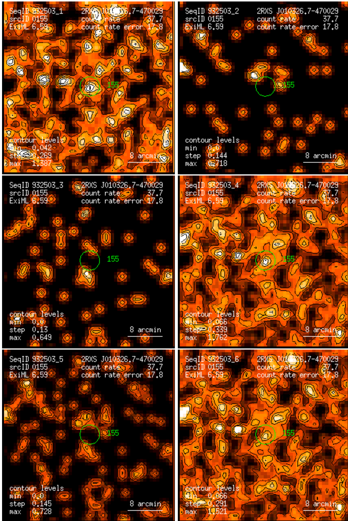
Figure 155: RASS 932503: detection 0155: band rate images, Gaussian filter: (1) PSPC channels 11 – 41, (2) 52 – 90, (3) 91 – 201, (4) 11 – 235, (5) 52 – 201, (6) 11 – 201. Broad band rates in counts/ks. Band rate contour levels in counts/ks/arcmin 2 .
