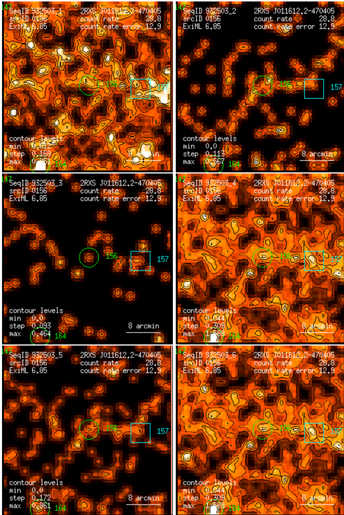
Figure 156: RASS 932503: detection 0156: band rate images, Gaussian filter: (1) PSPC channels 11 – 41, (2) 52 – 90, (3) 91 – 201, (4) 11 – 235, (5) 52 – 201, (6) 11 – 201. Broad band rates in counts/ks. Band rate contour levels in counts/ks/arcmin 2 .
