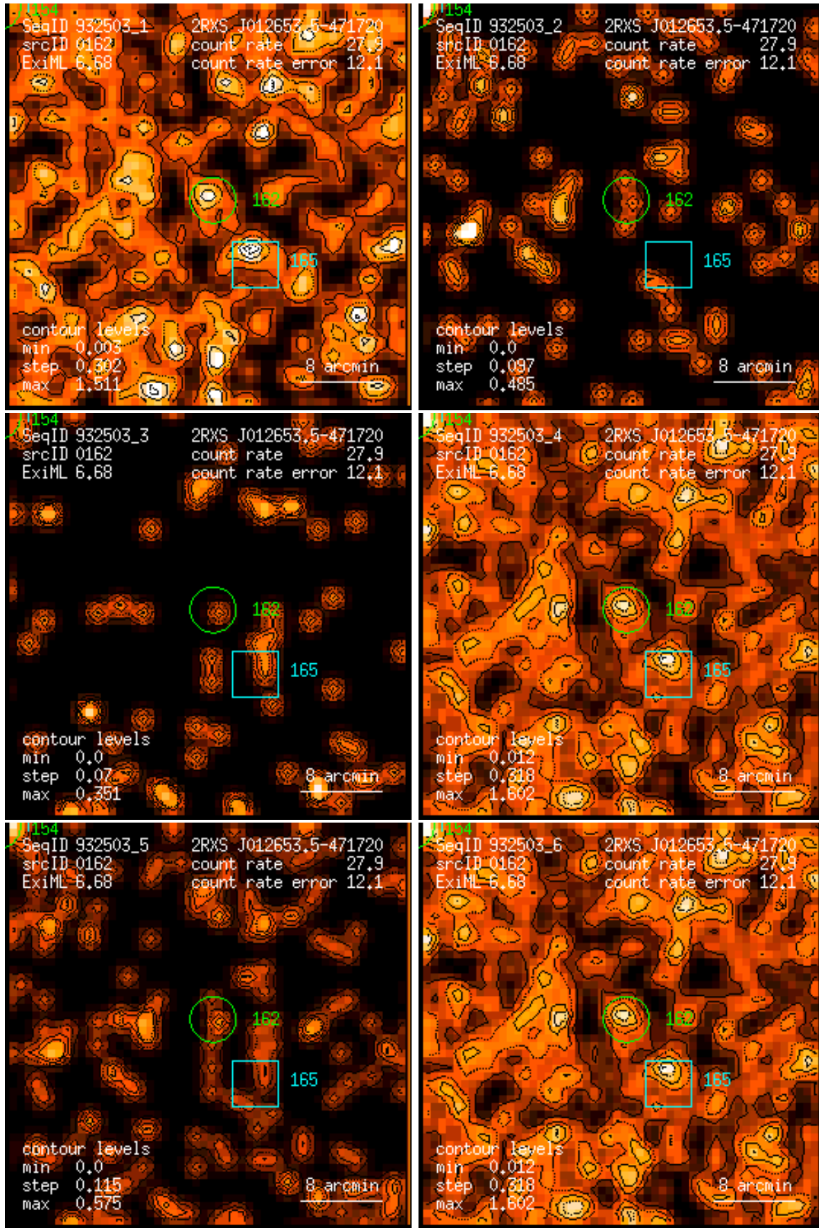
Figure 162: RASS 932503: detection 0162: band rate images, Gaussian filter: (1) PSPC channels 11 – 41, (2) 52 – 90, (3) 91 – 201, (4) 11 – 235, (5) 52 – 201, (6) 11 – 201. Broad band rates in counts/ks. Band rate contour levels in counts/ks/arcmin 2 .
