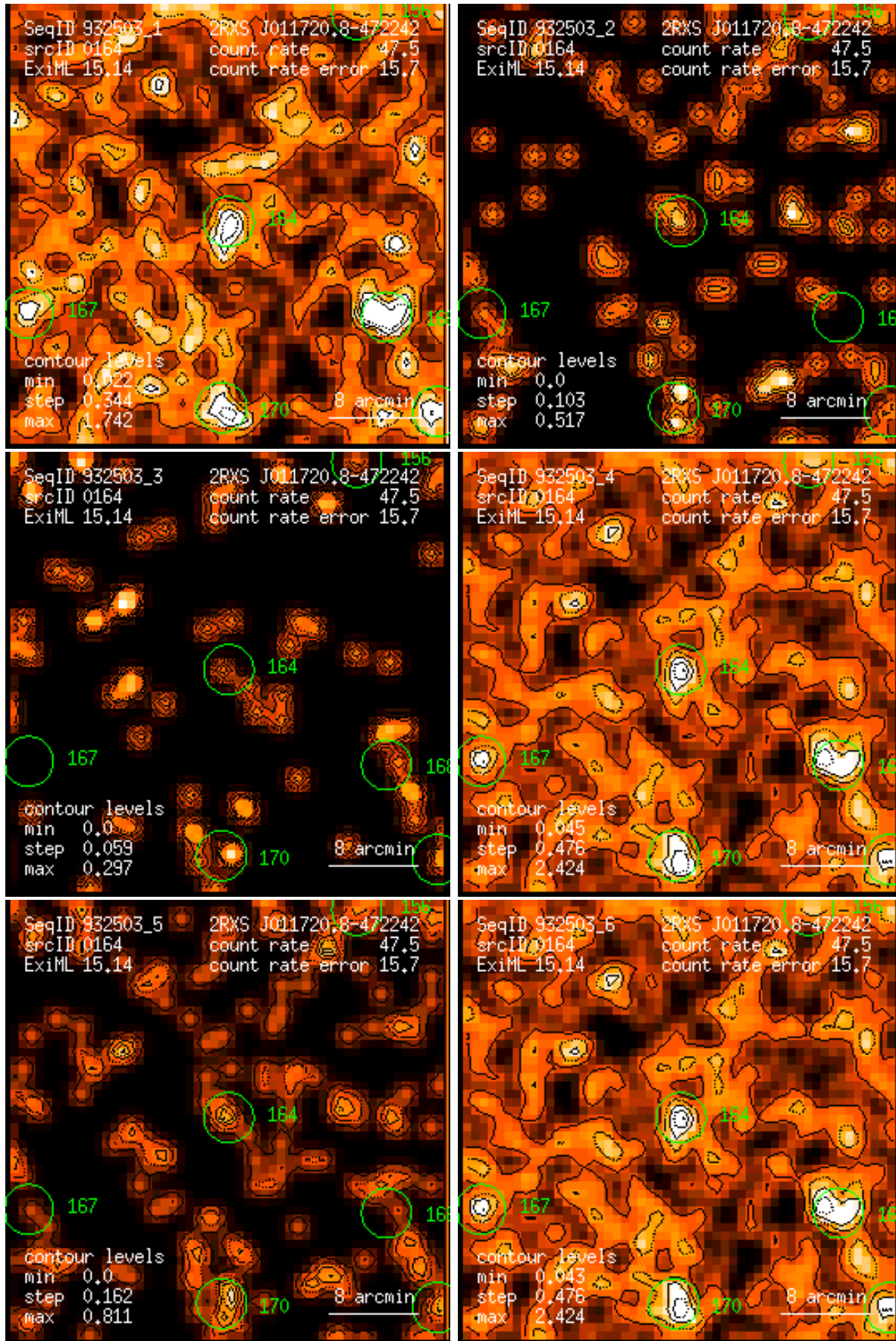
Figure 164: RASS 932503: detection 0164: band rate images, Gaussian filter: (1) PSPC channels 11 – 41, (2) 52 – 90, (3) 91 – 201, (4) 11 – 235, (5) 52 – 201, (6) 11 – 201. Broad band rates in counts/ks. Band rate contour levels in counts/ks/arcmin 2 .
