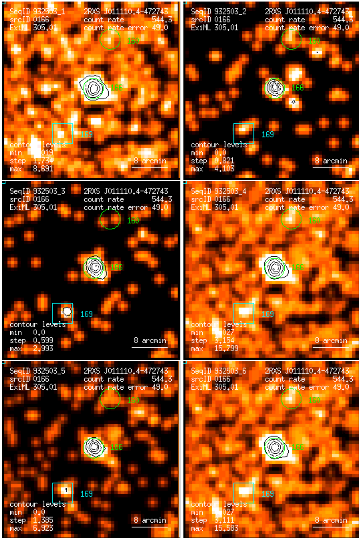
Figure 166: RASS 932503: detection 0166: band rate images, Gaussian filter: (1) PSPC channels 11 – 41, (2) 52 – 90, (3) 91 – 201, (4) 11 – 235, (5) 52 – 201, (6) 11 – 201. Broad band rates in counts/ks. Band rate contour levels in counts/ks/arcmin 2 .
