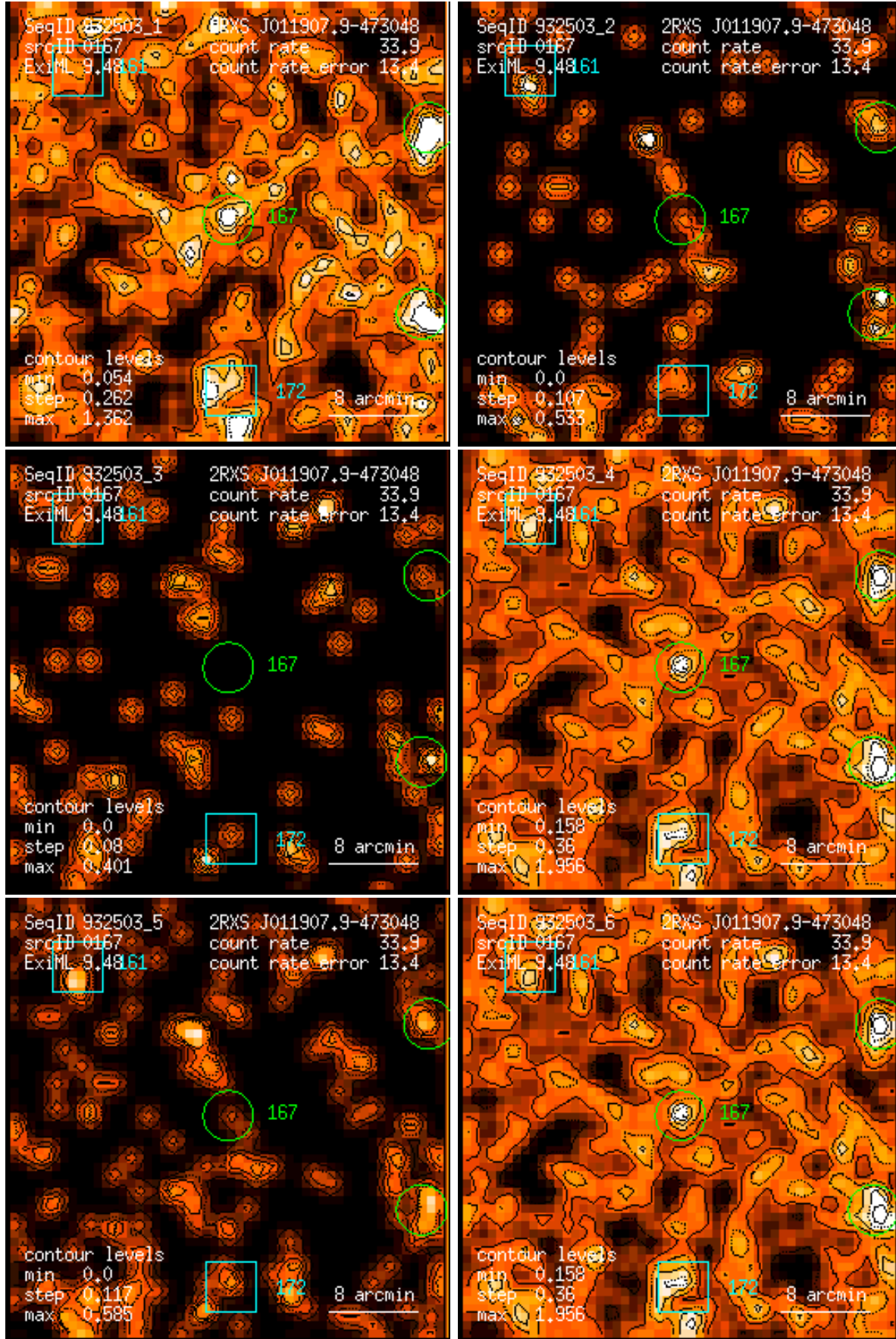
Figure 167: RASS 932503: detection 0167: band rate images, Gaussian filter: (1) PSPC channels 11 – 41, (2) 52 – 90, (3) 91 – 201, (4) 11 – 235, (5) 52 – 201, (6) 11 – 201. Broad band rates in counts/ks. Band rate contour levels in counts/ks/arcmin 2 .
