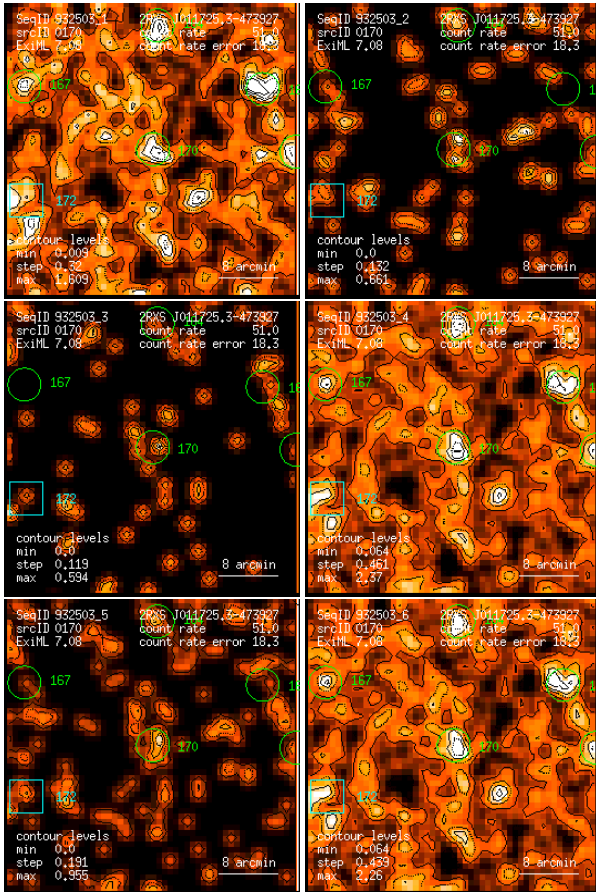
Figure 170: RASS 932503: detection 0170: band rate images, Gaussian filter: (1) PSPC channels 11 – 41, (2) 52 – 90, (3) 91 – 201, (4) 11 – 235, (5) 52 – 201, (6) 11 – 201. Broad band rates in counts/ks. Band rate contour levels in counts/ks/arcmin 2 .
