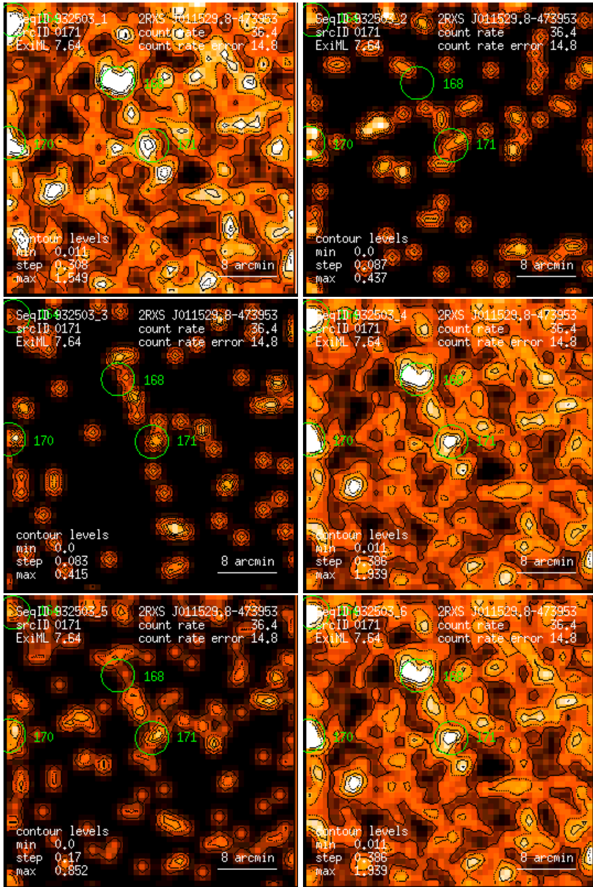
Figure 171: RASS 932503: detection 0171: band rate images, Gaussian filter: (1) PSPC channels 11 – 41, (2) 52 – 90, (3) 91 – 201, (4) 11 – 235, (5) 52 – 201, (6) 11 – 201. Broad band rates in counts/ks. Band rate contour levels in counts/ks/arcmin 2 .
