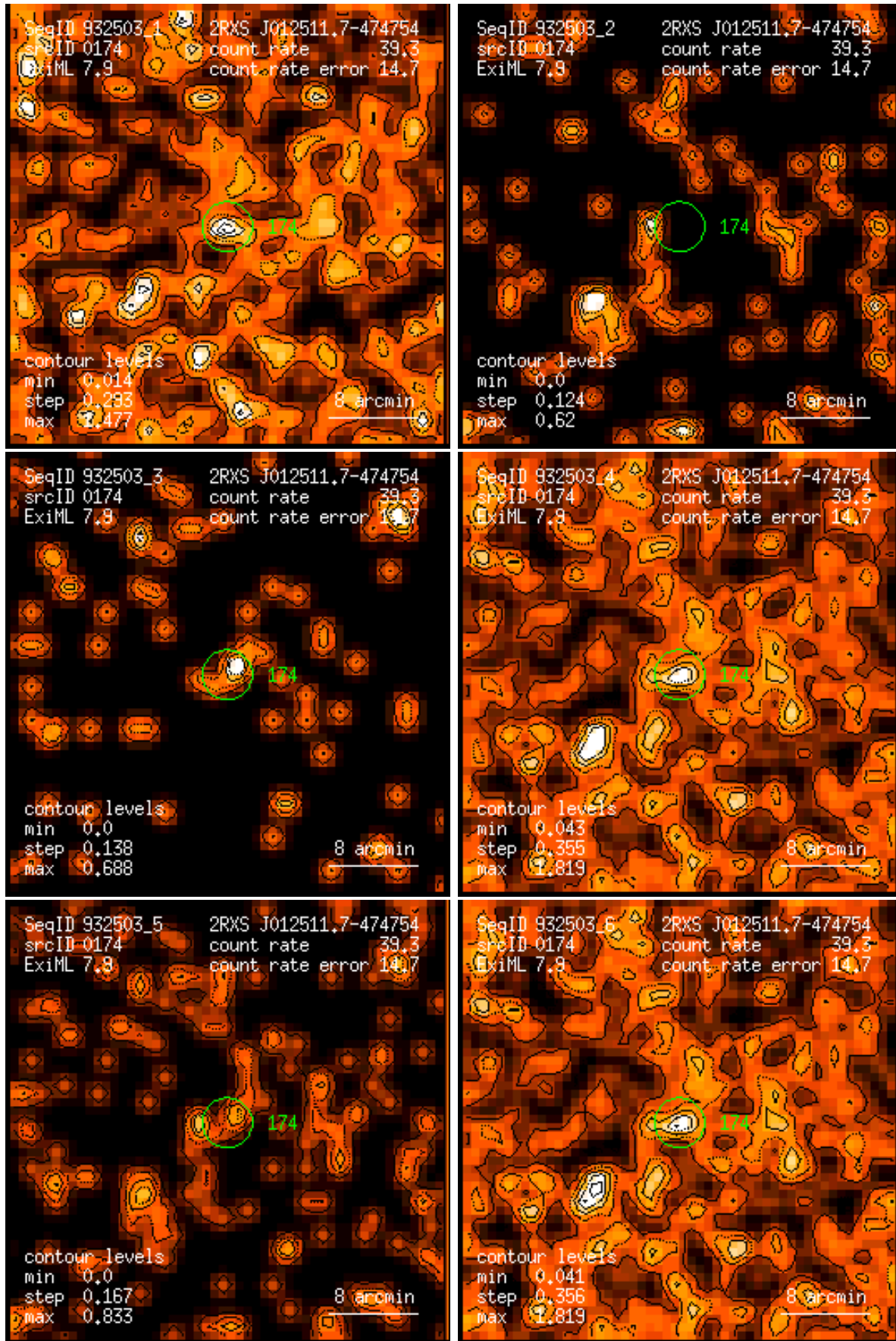
Figure 174: RASS 932503: detection 0174: band rate images, Gaussian filter: (1) PSPC channels 11 – 41, (2) 52 – 90, (3) 91 – 201, (4) 11 – 235, (5) 52 – 201, (6) 11 – 201. Broad band rates in counts/ks. Band rate contour levels in counts/ks/arcmin 2 .
