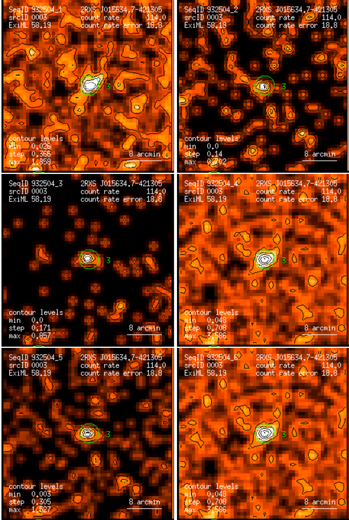
Figure 3: RASS 932504: detection 0003: band rate images, Gaussian filter: (1) PSPC channels 11 – 41, (2) 52 – 90, (3) 91 – 201, (4) 11 – 235, (5) 52 – 201, (6) 11 – 201. Broad band rates in counts/ks. Band rate contour levels in counts/ks/arcmin 2 .
