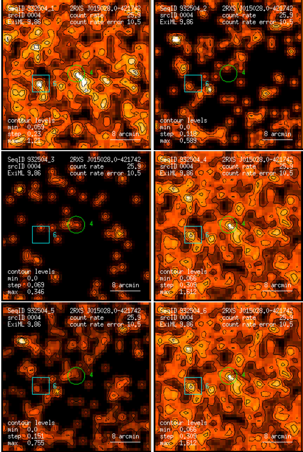
Figure 4: RASS 932504: detection 0004: band rate images, Gaussian filter: (1) PSPC channels 11 – 41, (2) 52 – 90, (3) 91 – 201, (4) 11 – 235, (5) 52 – 201, (6) 11 – 201. Broad band rates in counts/ks. Band rate contour levels in counts/ks/arcmin 2 .
