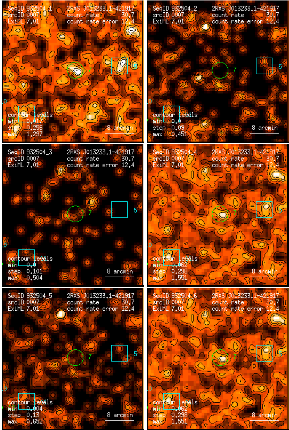
Figure 7: RASS 932504: detection 0007: band rate images, Gaussian filter: (1) PSPC channels 11 – 41, (2) 52 – 90, (3) 91 – 201, (4) 11 – 235, (5) 52 – 201, (6) 11 – 201. Broad band rates in counts/ks. Band rate contour levels in counts/ks/arcmin 2 .
