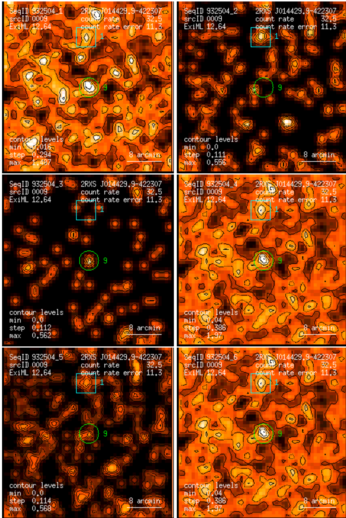
Figure 9: RASS 932504: detection 0009: band rate images, Gaussian filter: (1) PSPC channels 11 – 41, (2) 52 – 90, (3) 91 – 201, (4) 11 – 235, (5) 52 – 201, (6) 11 – 201. Broad band rates in counts/ks. Band rate contour levels in counts/ks/arcmin 2 .
