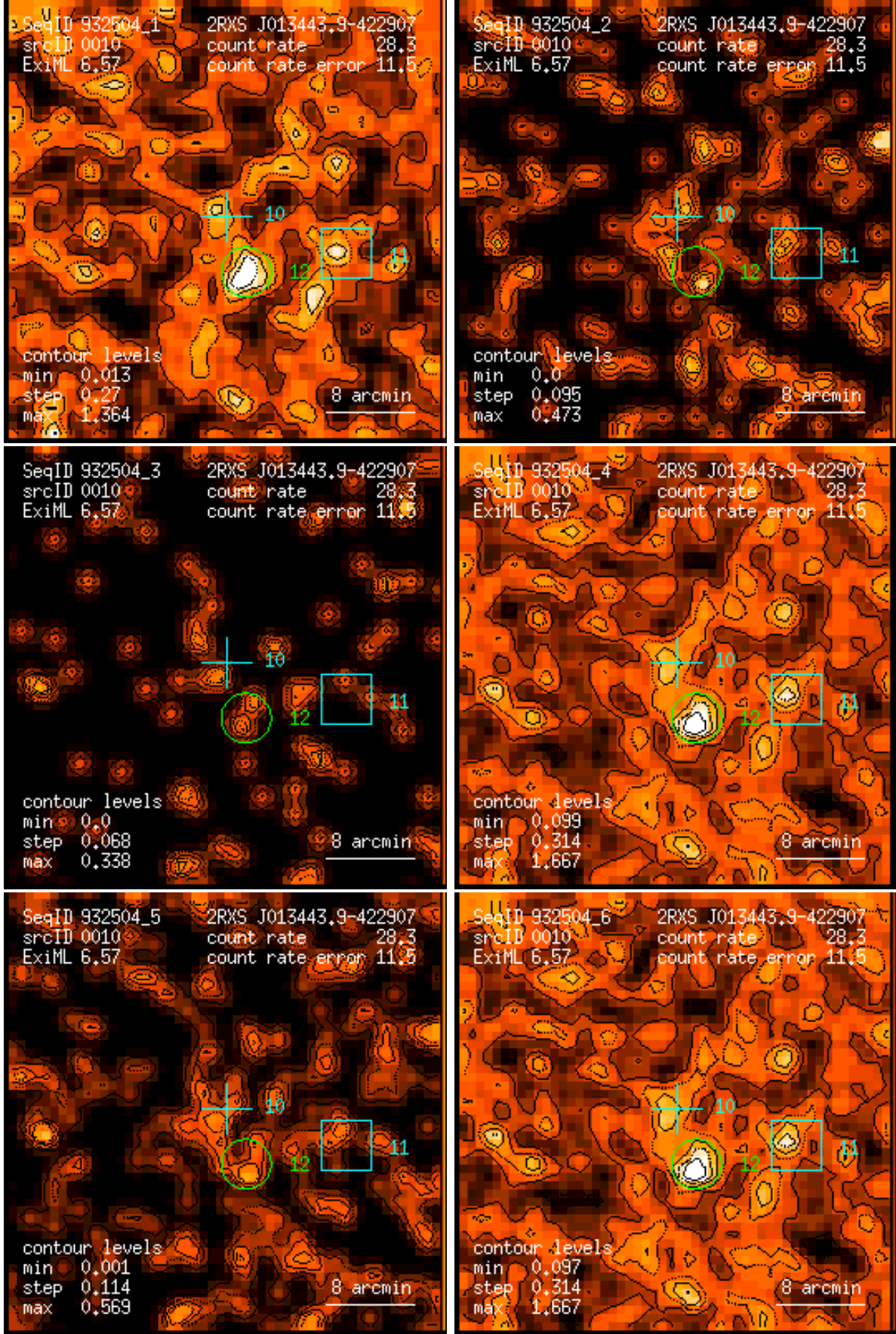
Figure 10: RASS 932504: detection 0010: band rate images, Gaussian filter: (1) PSPC channels 11 – 41, (2) 52 – 90, (3) 91 – 201, (4) 11 – 235, (5) 52 – 201, (6) 11 – 201. Broad band rates in counts/ks. Band rate contour levels in counts/ks/arcmin 2 .
