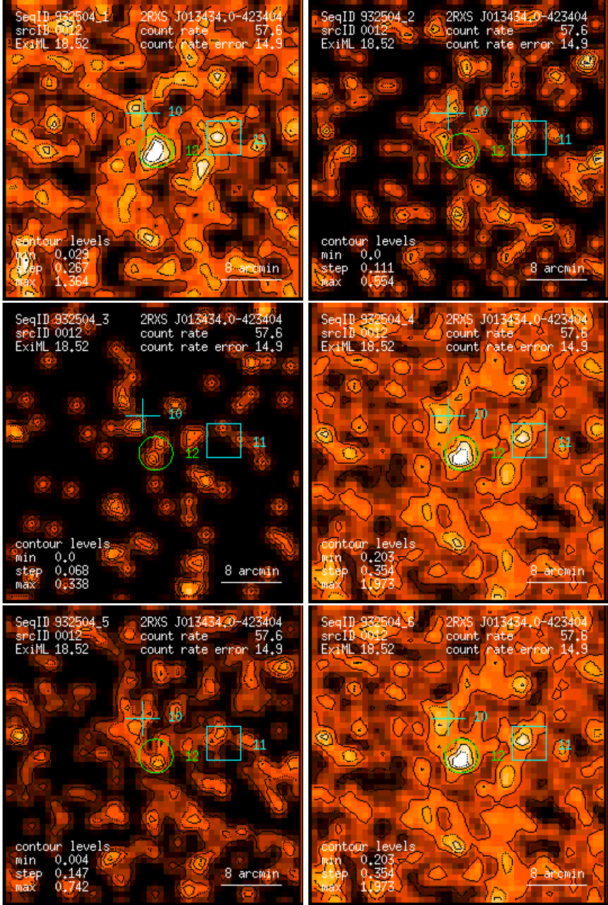
Figure 12: RASS 932504: detection 0012: band rate images, Gaussian filter: (1) PSPC channels 11 – 41, (2) 52 – 90, (3) 91 – 201, (4) 11 – 235, (5) 52 – 201, (6) 11 – 201. Broad band rates in counts/ks. Band rate contour levels in counts/ks/arcmin 2 .
