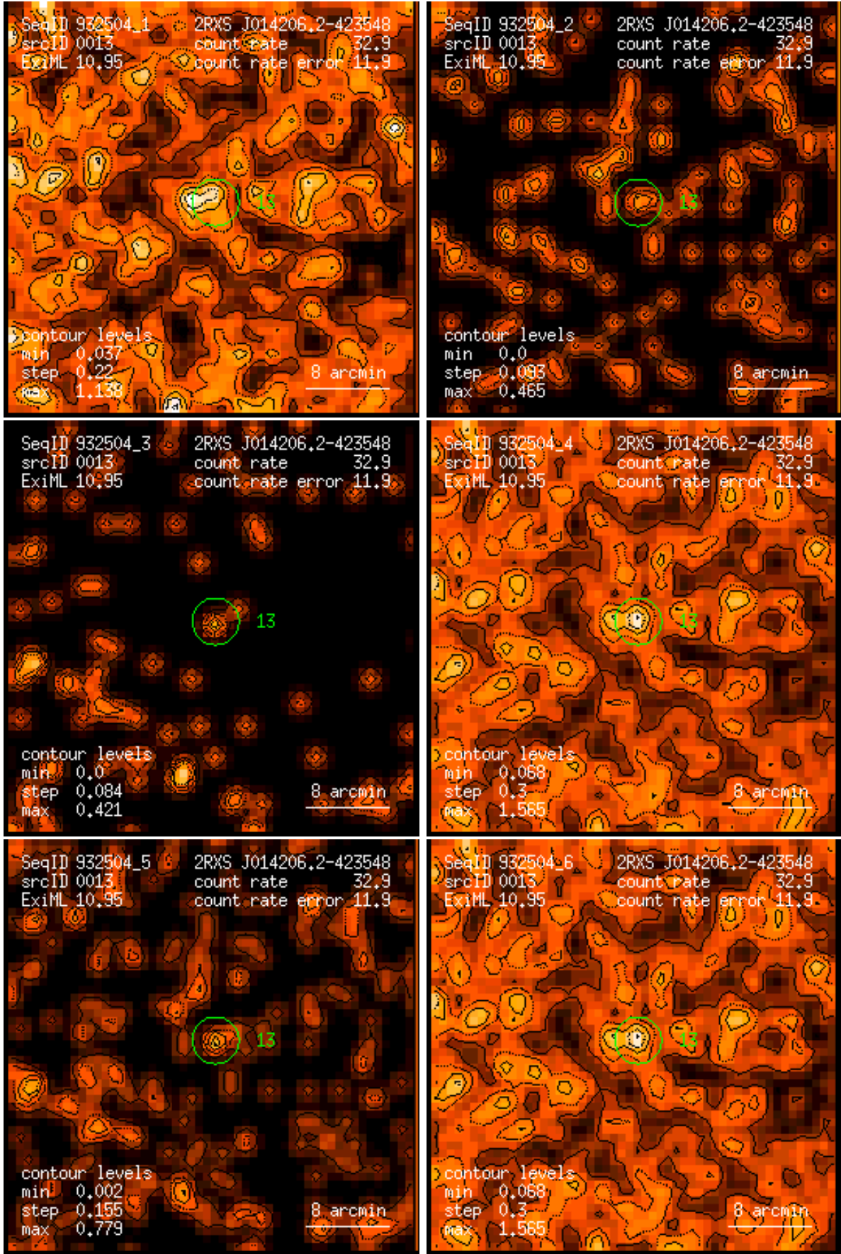
Figure 13: RASS 932504: detection 0013: band rate images, Gaussian filter: (1) PSPC channels 11 – 41, (2) 52 – 90, (3) 91 – 201, (4) 11 – 235, (5) 52 – 201, (6) 11 – 201. Broad band rates in counts/ks. Band rate contour levels in counts/ks/arcmin 2 .
