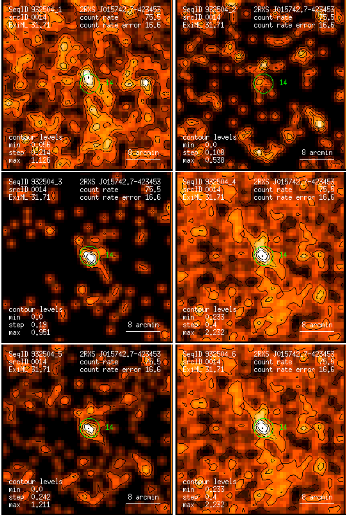
Figure 14: RASS 932504: detection 0014: band rate images, Gaussian filter: (1) PSPC channels 11 – 41, (2) 52 – 90, (3) 91 – 201, (4) 11 – 235, (5) 52 – 201, (6) 11 – 201. Broad band rates in counts/ks. Band rate contour levels in counts/ks/arcmin 2 .
