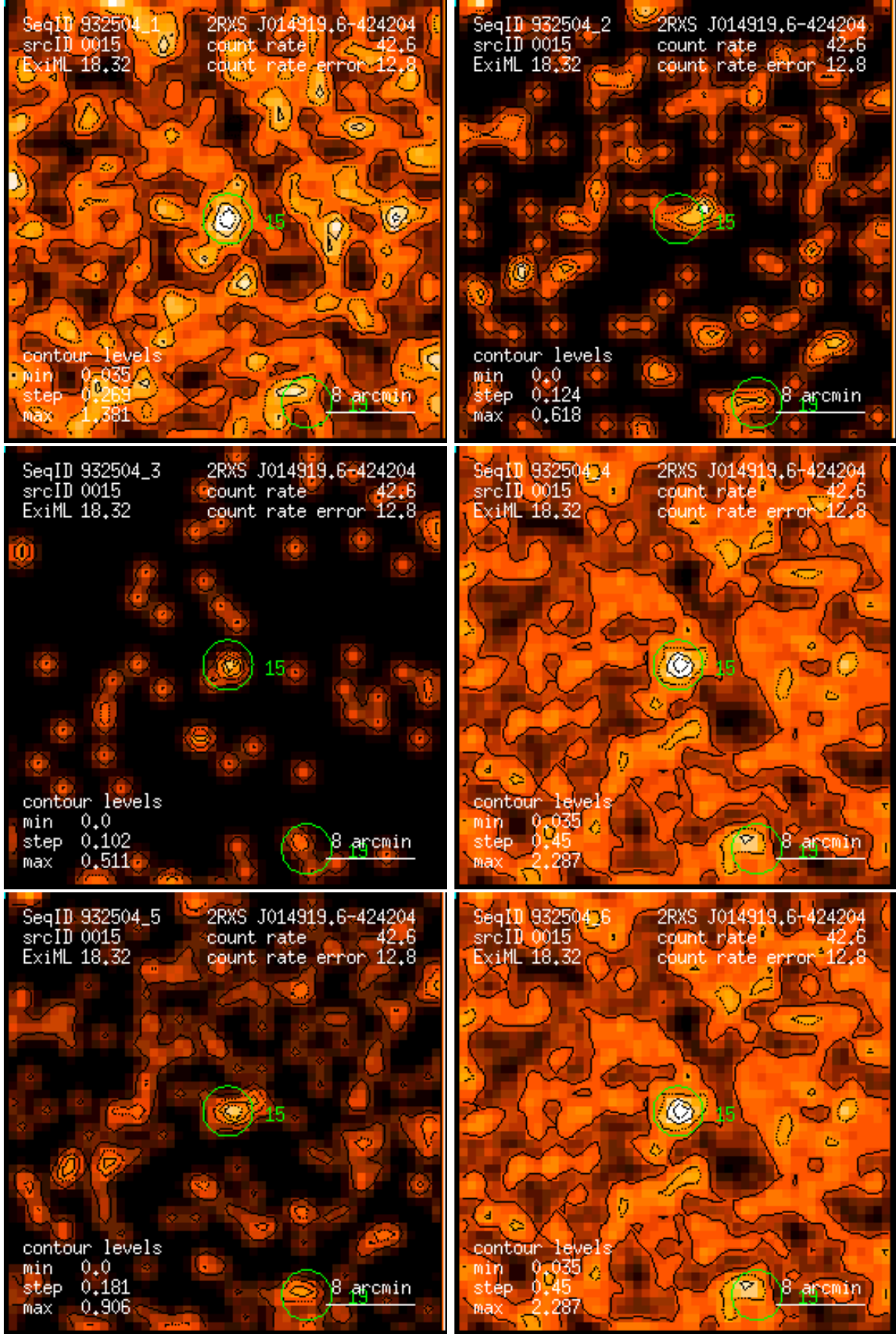
Figure 15: RASS 932504: detection 0015: band rate images, Gaussian filter: (1) PSPC channels 11 – 41, (2) 52 – 90, (3) 91 – 201, (4) 11 – 235, (5) 52 – 201, (6) 11 – 201. Broad band rates in counts/ks. Band rate contour levels in counts/ks/arcmin 2 .
