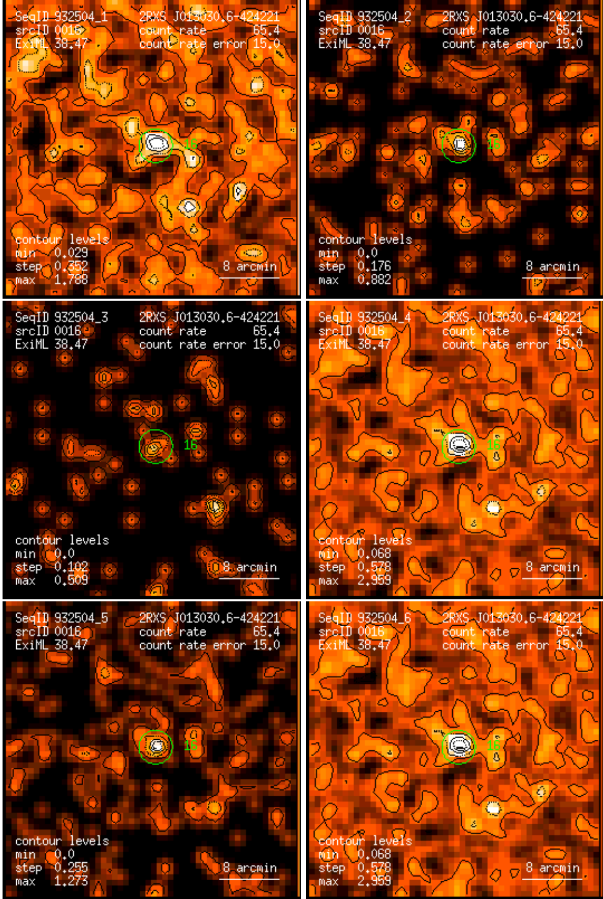
Figure 16: RASS 932504: detection 0016: band rate images, Gaussian filter: (1) PSPC channels 11 – 41, (2) 52 – 90, (3) 91 – 201, (4) 11 – 235, (5) 52 – 201, (6) 11 – 201. Broad band rates in counts/ks. Band rate contour levels in counts/ks/arcmin 2 .
