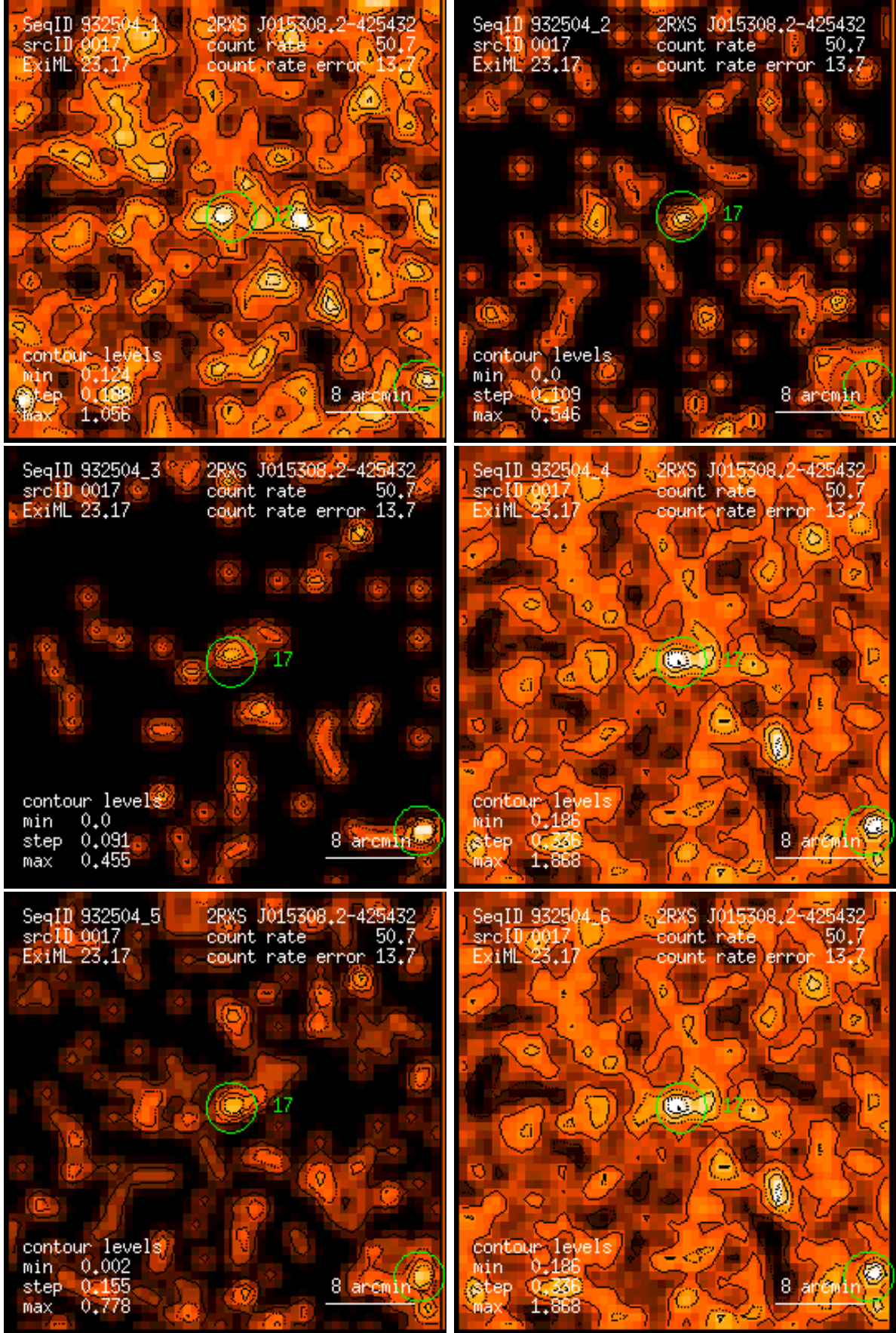
Figure 17: RASS 932504: detection 0017: band rate images, Gaussian filter: (1) PSPC channels 11 – 41, (2) 52 – 90, (3) 91 – 201, (4) 11 – 235, (5) 52 – 201, (6) 11 – 201. Broad band rates in counts/ks. Band rate contour levels in counts/ks/arcmin 2 .
