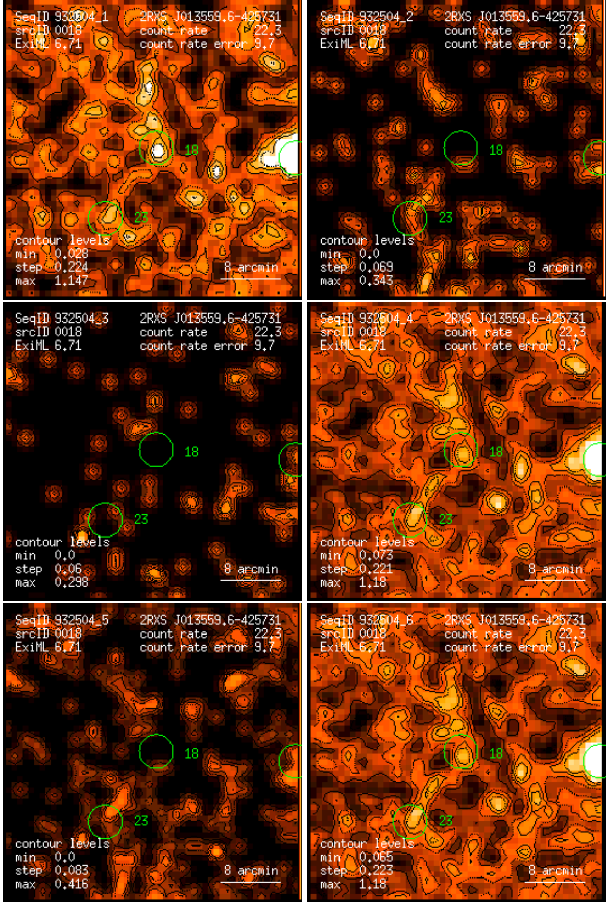
Figure 18: RASS 932504: detection 0018: band rate images, Gaussian filter: (1) PSPC channels 11 – 41, (2) 52 – 90, (3) 91 – 201, (4) 11 – 235, (5) 52 – 201, (6) 11 – 201. Broad band rates in counts/ks. Band rate contour levels in counts/ks/arcmin 2 .
