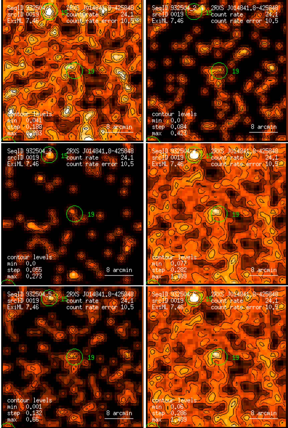
Figure 19: RASS 932504: detection 0019: band rate images, Gaussian filter: (1) PSPC channels 11 – 41, (2) 52 – 90, (3) 91 – 201, (4) 11 – 235, (5) 52 – 201, (6) 11 – 201. Broad band rates in counts/ks. Band rate contour levels in counts/ks/arcmin 2 .
