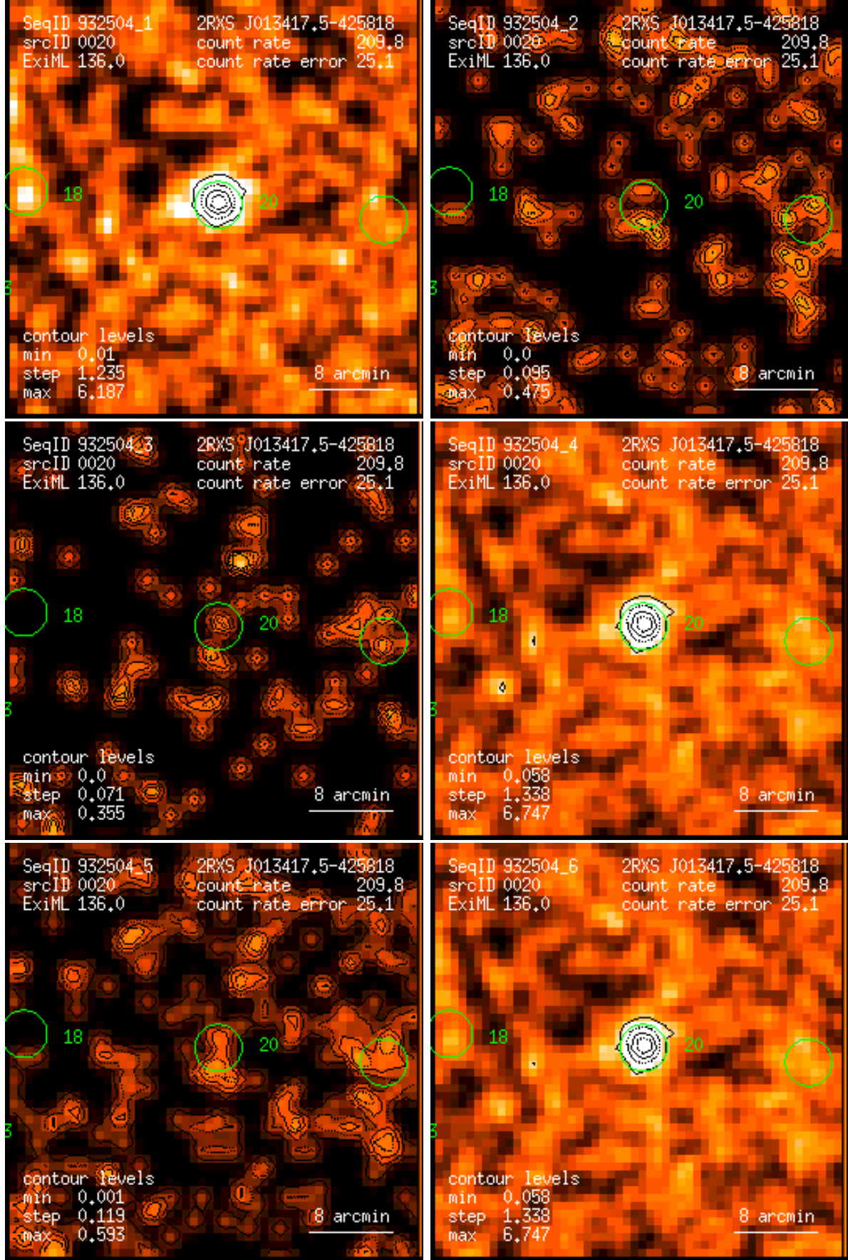
Figure 20: RASS 932504: detection 0020: band rate images, Gaussian filter: (1) PSPC channels 11 – 41, (2) 52 – 90, (3) 91 – 201, (4) 11 – 235, (5) 52 – 201, (6) 11 – 201. Broad band rates in counts/ks. Band rate contour levels in counts/ks/arcmin 2 .
