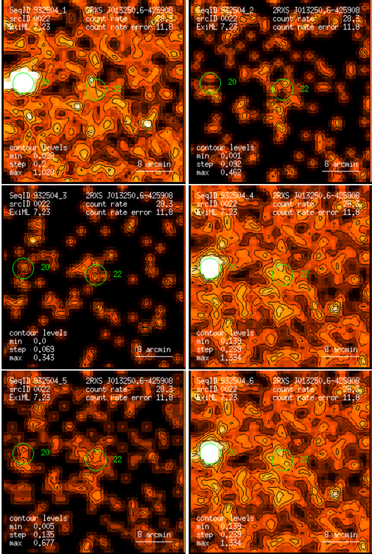
Figure 22: RASS 932504: detection 0022: band rate images, Gaussian filter: (1) PSPC channels 11 – 41, (2) 52 – 90, (3) 91 – 201, (4) 11 – 235, (5) 52 – 201, (6) 11 – 201. Broad band rates in counts/ks. Band rate contour levels in counts/ks/arcmin 2 .
