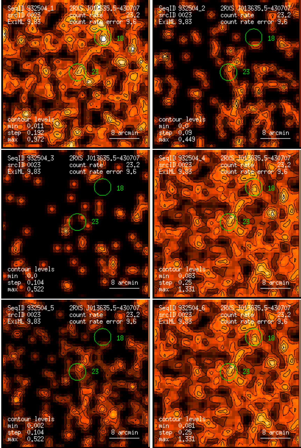
Figure 23: RASS 932504: detection 0023: band rate images, Gaussian filter: (1) PSPC channels 11 – 41, (2) 52 – 90, (3) 91 – 201, (4) 11 – 235, (5) 52 – 201, (6) 11 – 201. Broad band rates in counts/ks. Band rate contour levels in counts/ks/arcmin 2 .
