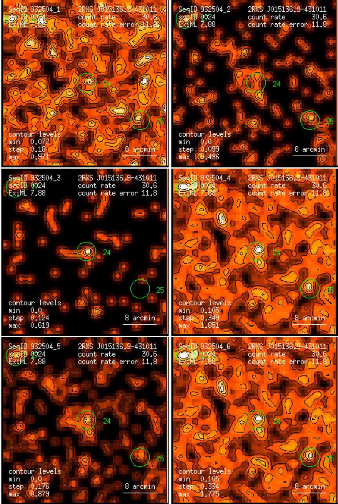
Figure 24: RASS 932504: detection 0024: band rate images, Gaussian filter: (1) PSPC channels 11 – 41, (2) 52 – 90, (3) 91 – 201, (4) 11 – 235, (5) 52 – 201, (6) 11 – 201. Broad band rates in counts/ks. Band rate contour levels in counts/ks/arcmin 2 .
