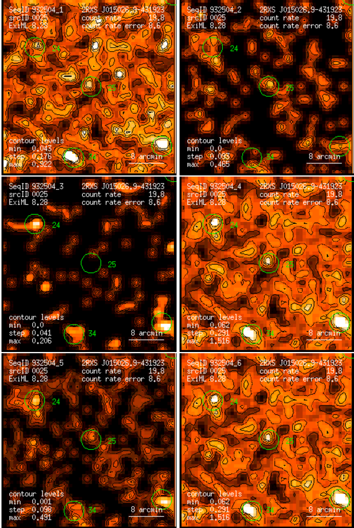
Figure 25: RASS 932504: detection 0025: band rate images, Gaussian filter: (1) PSPC channels 11 – 41, (2) 52 – 90, (3) 91 – 201, (4) 11 – 235, (5) 52 – 201, (6) 11 – 201. Broad band rates in counts/ks. Band rate contour levels in counts/ks/arcmin 2 .
