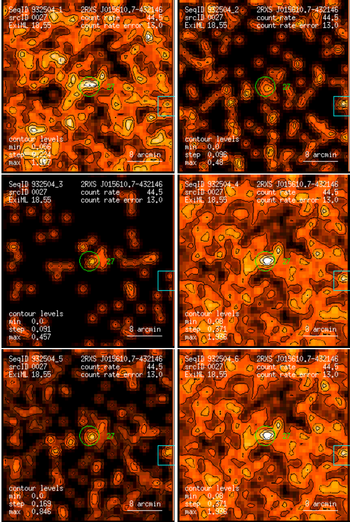
Figure 27: RASS 932504: detection 0027: band rate images, Gaussian filter: (1) PSPC channels 11 – 41, (2) 52 – 90, (3) 91 – 201, (4) 11 – 235, (5) 52 – 201, (6) 11 – 201. Broad band rates in counts/ks. Band rate contour levels in counts/ks/arcmin 2 .
