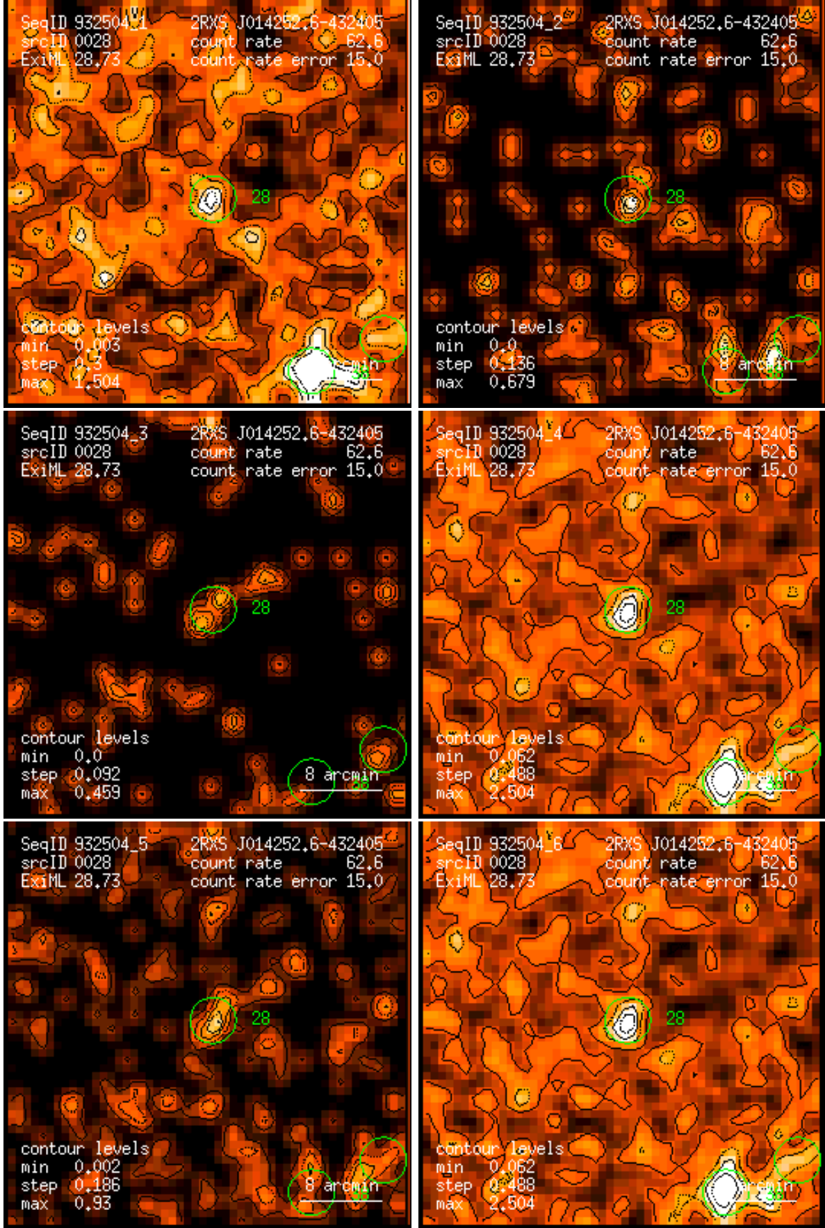
Figure 28: RASS 932504: detection 0028: band rate images, Gaussian filter: (1) PSPC channels 11 – 41, (2) 52 – 90, (3) 91 – 201, (4) 11 – 235, (5) 52 – 201, (6) 11 – 201. Broad band rates in counts/ks. Band rate contour levels in counts/ks/arcmin 2 .
