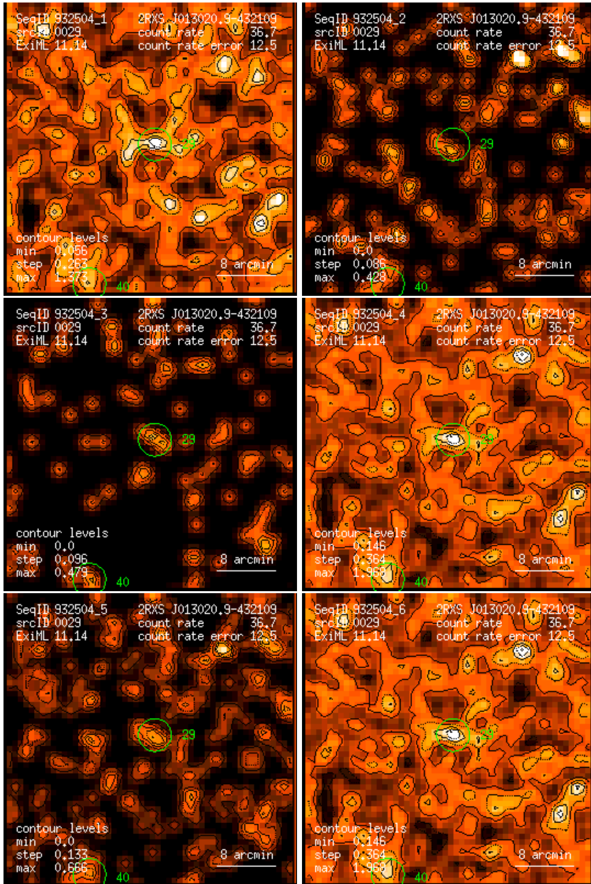
Figure 29: RASS 932504: detection 0029: band rate images, Gaussian filter: (1) PSPC channels 11 – 41, (2) 52 – 90, (3) 91 – 201, (4) 11 – 235, (5) 52 – 201, (6) 11 – 201. Broad band rates in counts/ks. Band rate contour levels in counts/ks/arcmin 2 .
