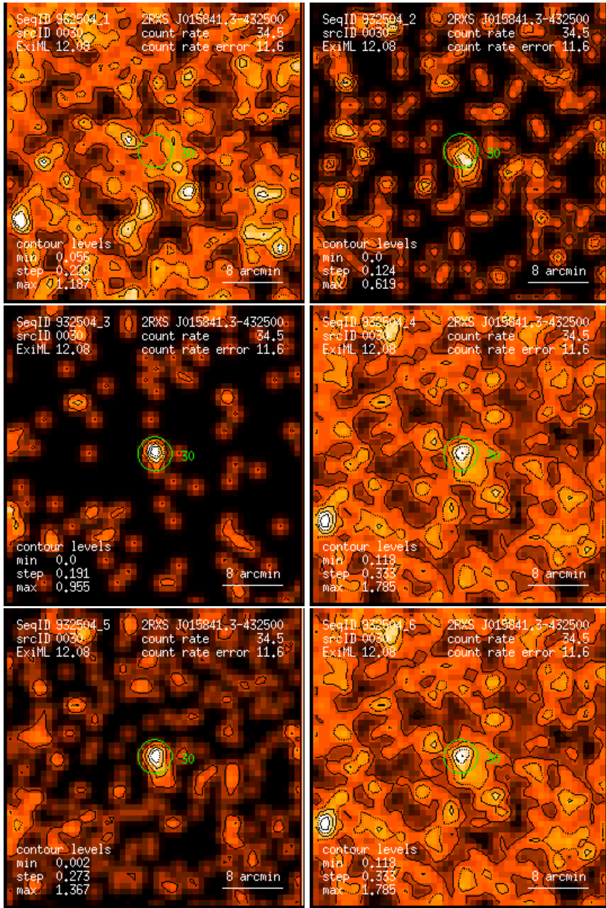
Figure 30: RASS 932504: detection 0030: band rate images, Gaussian filter: (1) PSPC channels 11 – 41, (2) 52 – 90, (3) 91 – 201, (4) 11 – 235, (5) 52 – 201, (6) 11 – 201. Broad band rates in counts/ks. Band rate contour levels in counts/ks/arcmin 2 .
