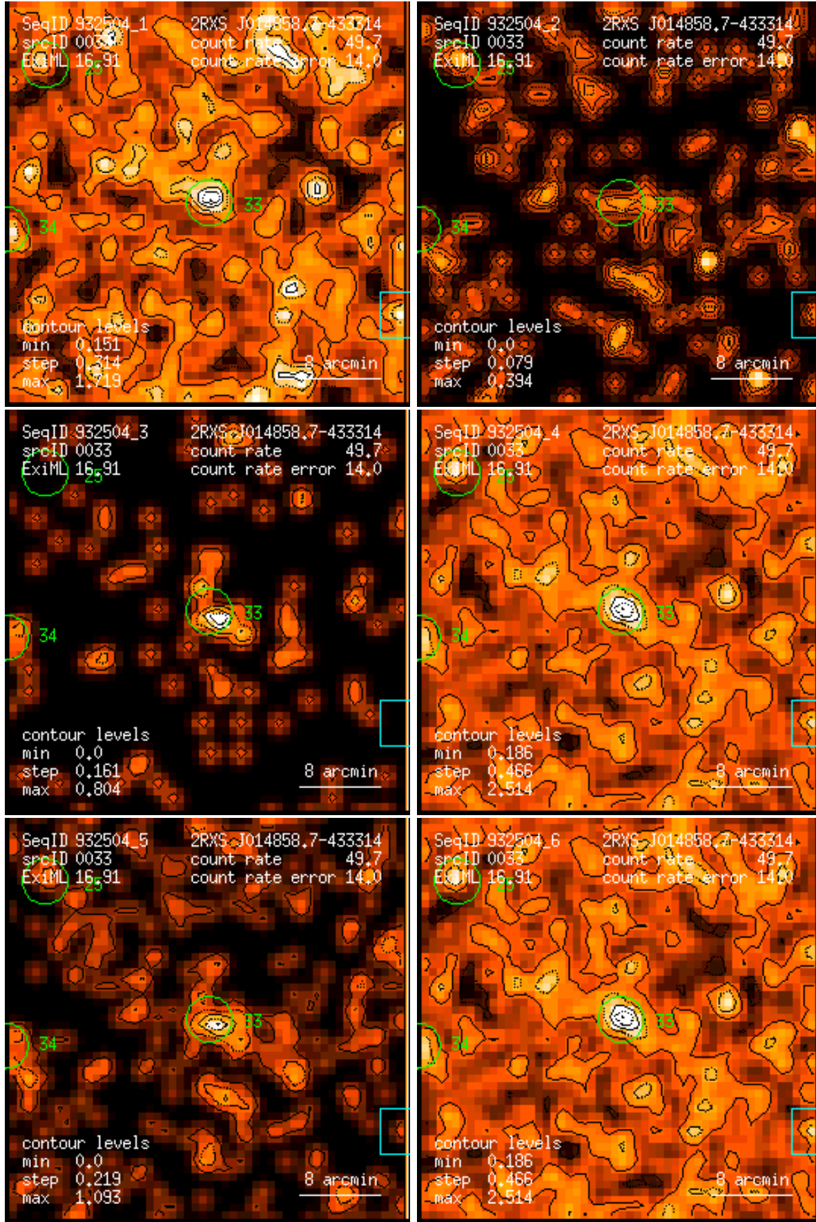
Figure 33: RASS 932504: detection 0033: band rate images, Gaussian filter: (1) PSPC channels 11 – 41, (2) 52 – 90, (3) 91 – 201, (4) 11 – 235, (5) 52 – 201, (6) 11 – 201. Broad band rates in counts/ks. Band rate contour levels in counts/ks/arcmin 2 .
