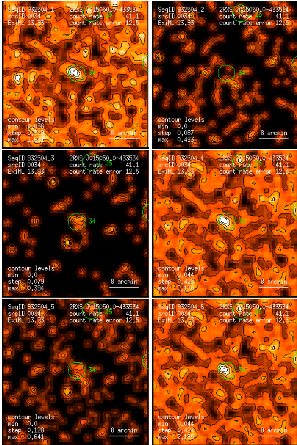
Figure 34: RASS 932504: detection 0034: band rate images, Gaussian filter: (1) PSPC channels 11 – 41, (2) 52 – 90, (3) 91 – 201, (4) 11 – 235, (5) 52 – 201, (6) 11 – 201. Broad band rates in counts/ks. Band rate contour levels in counts/ks/arcmin 2 .
