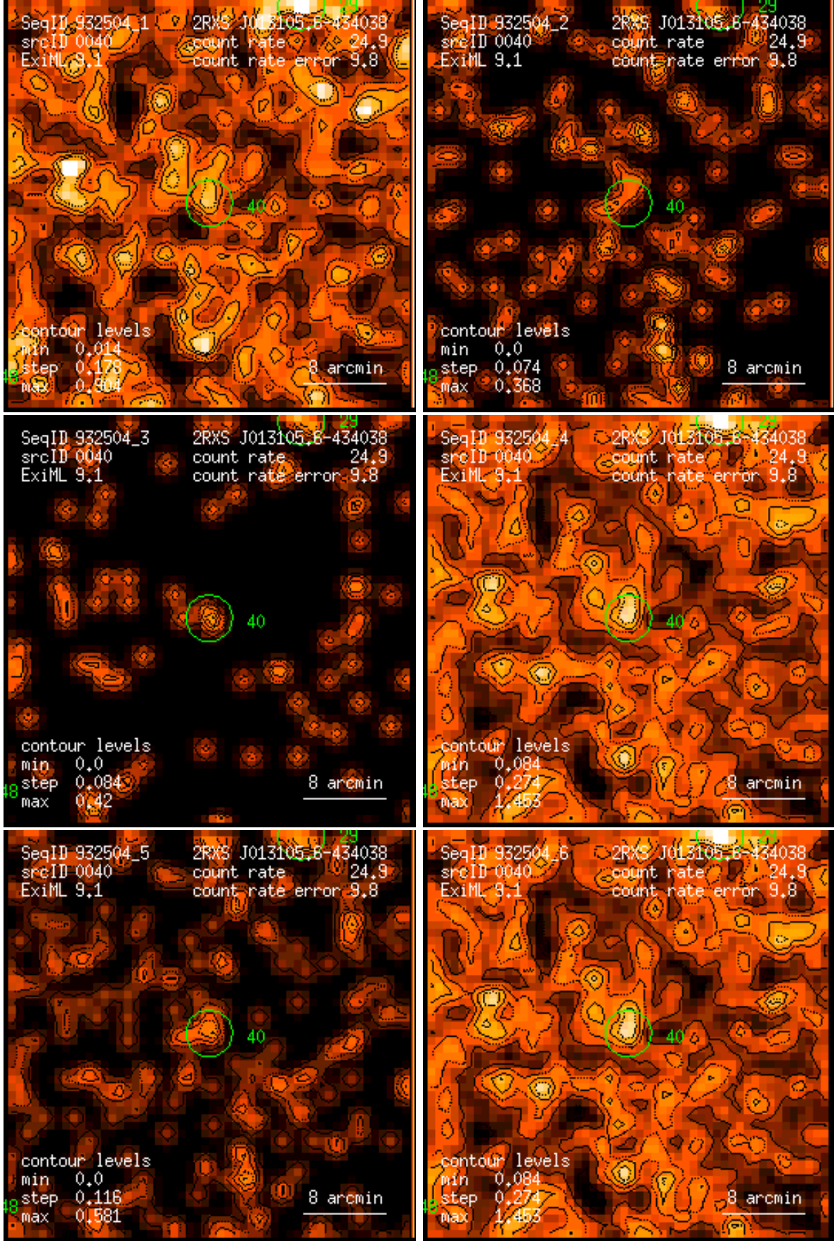
Figure 40: RASS 932504: detection 0040: band rate images, Gaussian filter: (1) PSPC channels 11 – 41, (2) 52 – 90, (3) 91 – 201, (4) 11 – 235, (5) 52 – 201, (6) 11 – 201. Broad band rates in counts/ks. Band rate contour levels in counts/ks/arcmin 2 .
