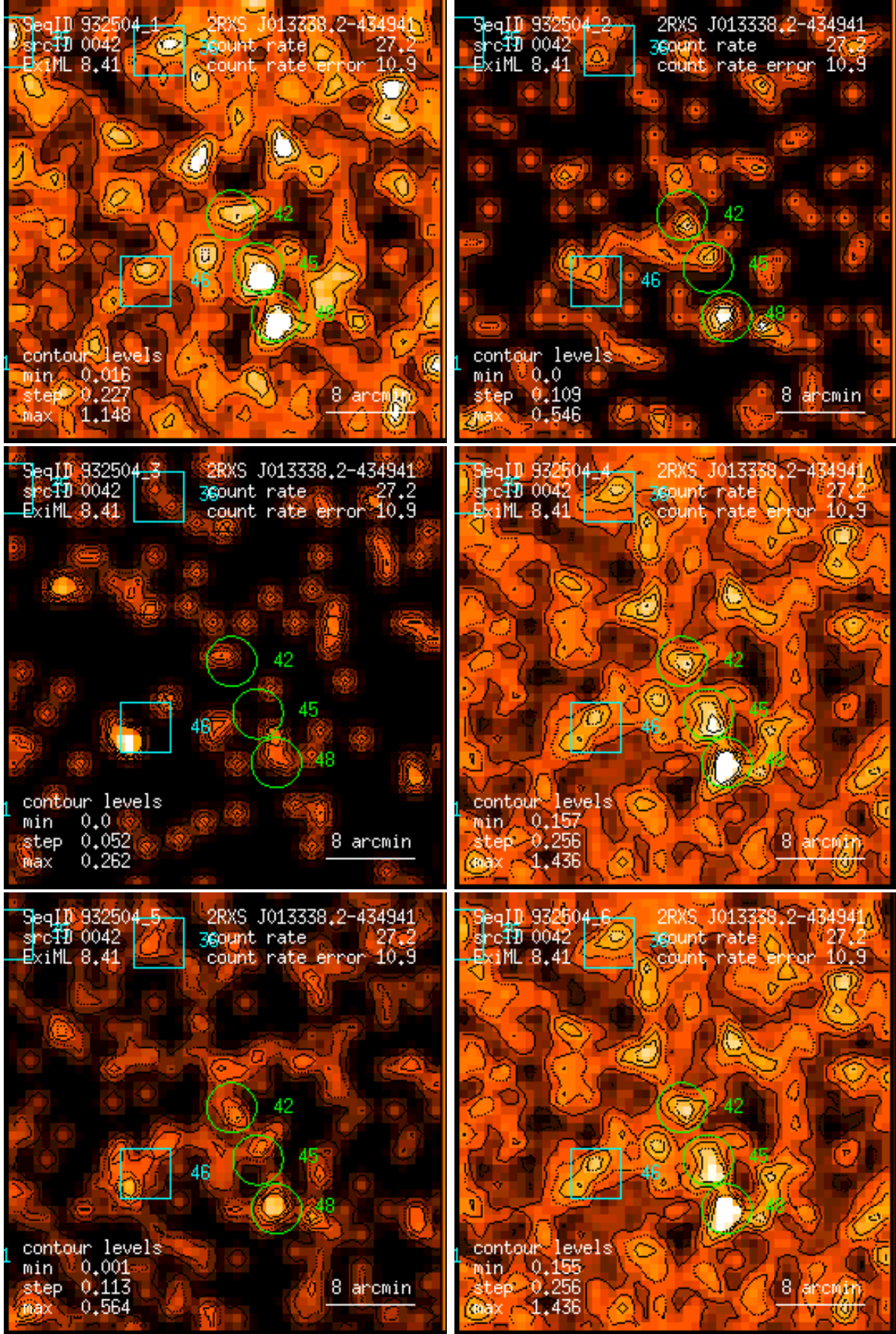
Figure 42: RASS 932504: detection 0042: band rate images, Gaussian filter: (1) PSPC channels 11 – 41, (2) 52 – 90, (3) 91 – 201, (4) 11 – 235, (5) 52 – 201, (6) 11 – 201. Broad band rates in counts/ks. Band rate contour levels in counts/ks/arcmin 2 .
