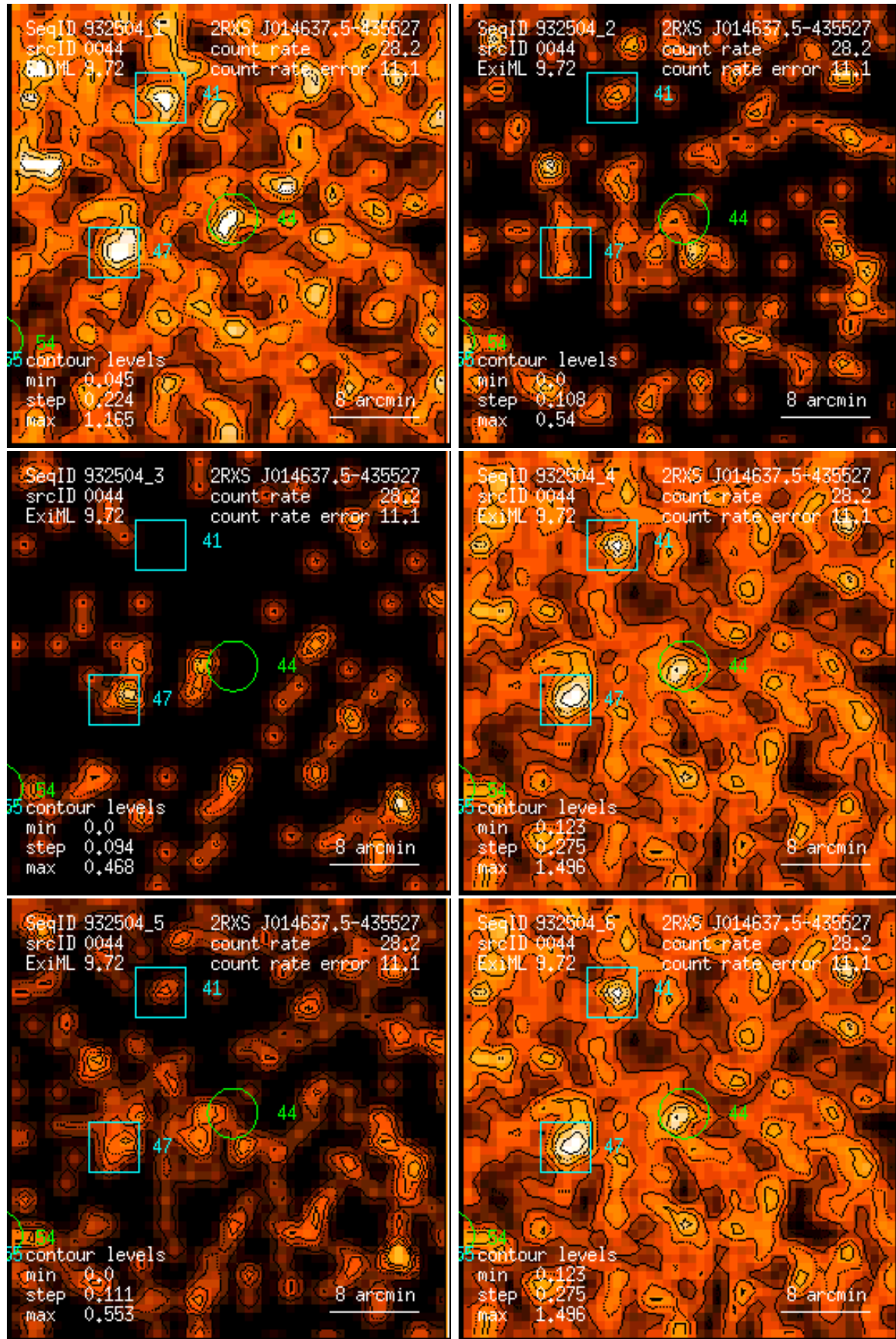
Figure 44: RASS 932504: detection 0044: band rate images, Gaussian filter: (1) PSPC channels 11 – 41, (2) 52 – 90, (3) 91 – 201, (4) 11 – 235, (5) 52 – 201, (6) 11 – 201. Broad band rates in counts/ks. Band rate contour levels in counts/ks/arcmin 2 .
