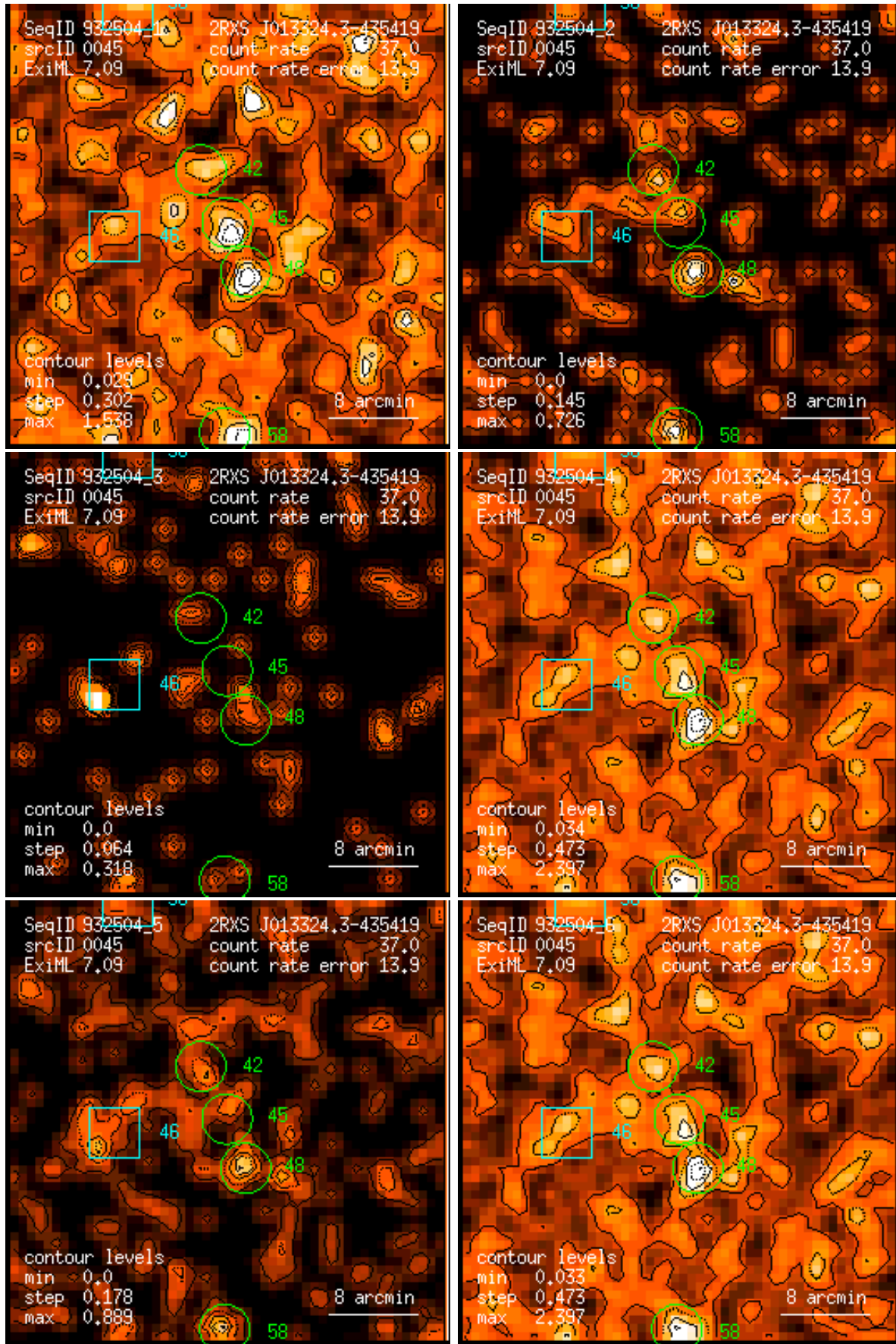
Figure 45: RASS 932504: detection 0045: band rate images, Gaussian filter: (1) PSPC channels 11 – 41, (2) 52 – 90, (3) 91 – 201, (4) 11 – 235, (5) 52 – 201, (6) 11 – 201. Broad band rates in counts/ks. Band rate contour levels in counts/ks/arcmin 2 .
