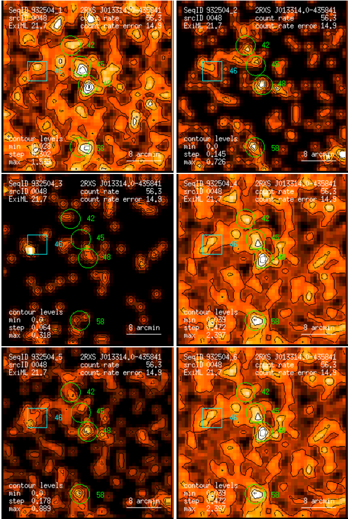
Figure 48: RASS 932504: detection 0048: band rate images, Gaussian filter: (1) PSPC channels 11 – 41, (2) 52 – 90, (3) 91 – 201, (4) 11 – 235, (5) 52 – 201, (6) 11 – 201. Broad band rates in counts/ks. Band rate contour levels in counts/ks/arcmin 2 .
