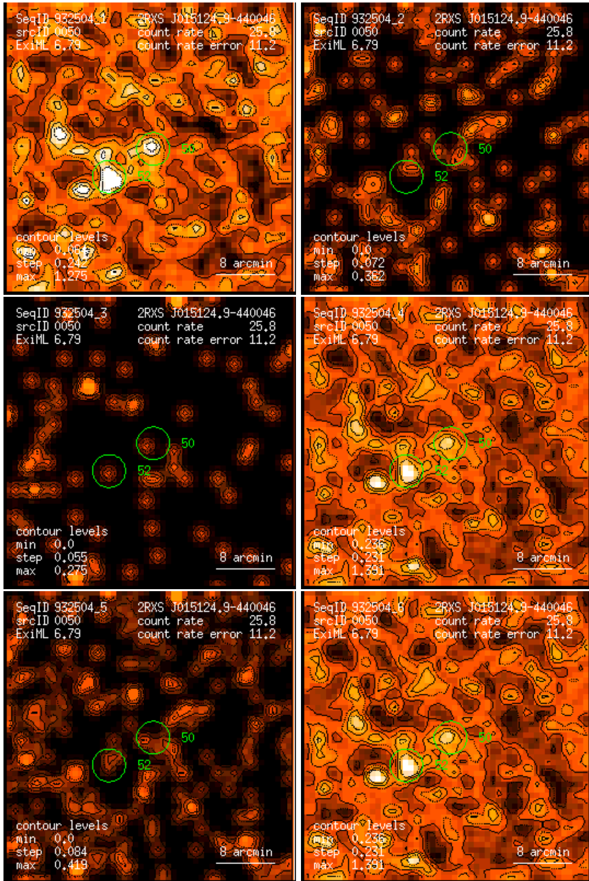
Figure 50: RASS 932504: detection 0050: band rate images, Gaussian filter: (1) PSPC channels 11 – 41, (2) 52 – 90, (3) 91 – 201, (4) 11 – 235, (5) 52 – 201, (6) 11 – 201. Broad band rates in counts/ks. Band rate contour levels in counts/ks/arcmin 2 .
