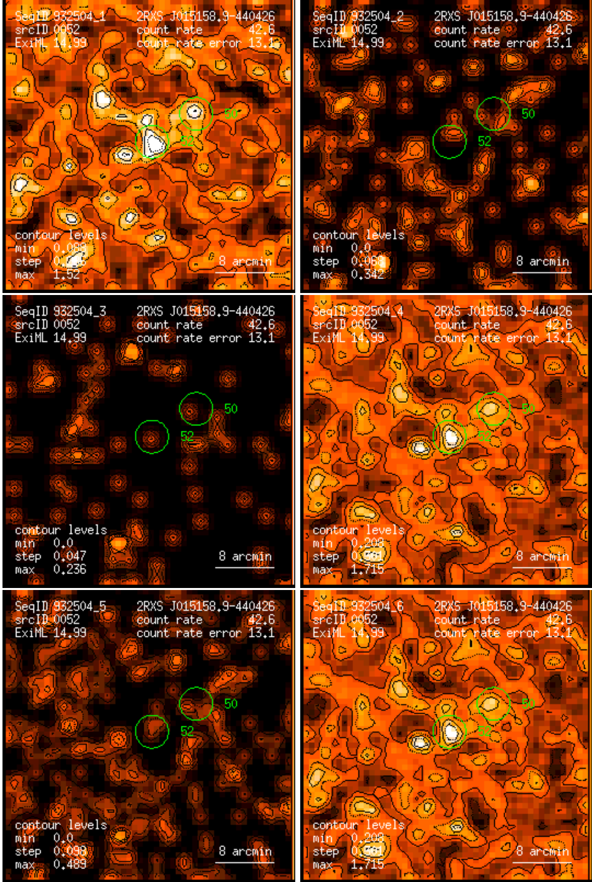
Figure 52: RASS 932504: detection 0052: band rate images, Gaussian filter: (1) PSPC channels 11 – 41, (2) 52 – 90, (3) 91 – 201, (4) 11 – 235, (5) 52 – 201, (6) 11 – 201. Broad band rates in counts/ks. Band rate contour levels in counts/ks/arcmin 2 .
